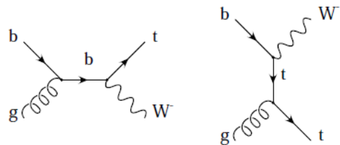
Figure 1: Leading-order Feynman diagrams for associated production of a single top-quark and a W boson.
