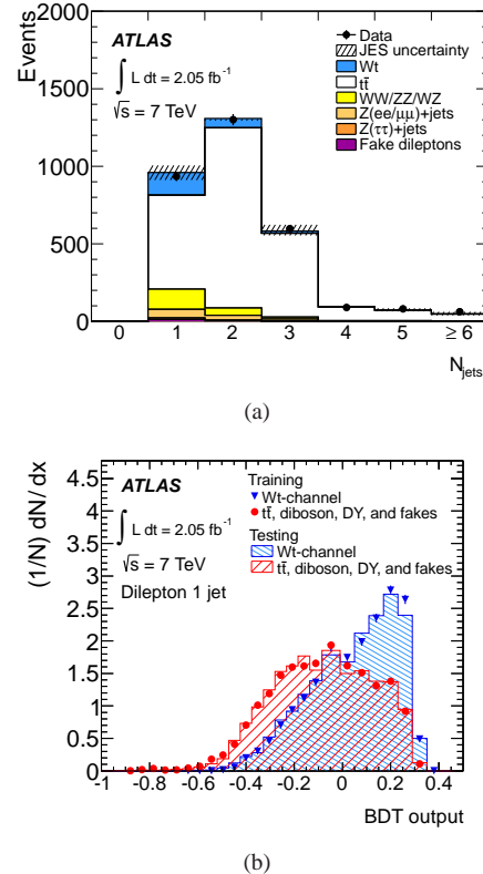
Figure 2: (a) Number of jets with p_T > 30 GeV and |\eta| < 2.5 after the selection; hatched bands show the jet energy scale (JES) uncertainty. The Wt signal is normalised to the theory prediction. (b) Distribution of BDT output for the signal ( Wt -channel) and background ( t\bar{t} diboson, Drell-Yan and fake dileptons) in signal enriched 1-jet bin. The BDT method uses 2 statistically independent sets of MC-simulated events, indicated as training and testing samples, to check both signal and background BDT output stability. The BDT weight file is derived from a training sample and applied to a testing sample.
