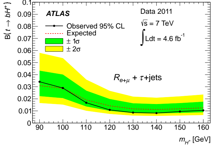
Figure 6. Upper limits on \mathcal{B}(t \rightarrow bH^+) derived from the transverse mass distribution of \tau_{\text{had}}+\text{jets} events in ref. [8] and the event yield ratio R_{e+\mu} , as a function of the charged Higgs boson mass, obtained for an integrated luminosity of 4.6 \text{ fb}^{-1} and with the assumption \mathcal{B}(H^+ \rightarrow \tau\nu) = 1 . The solid line in the figure is used to denote the observed 95% CL upper limits, while the dashed line represents the expected exclusion limits. The green and yellow regions show the 1\sigma and 2\sigma error bands.
