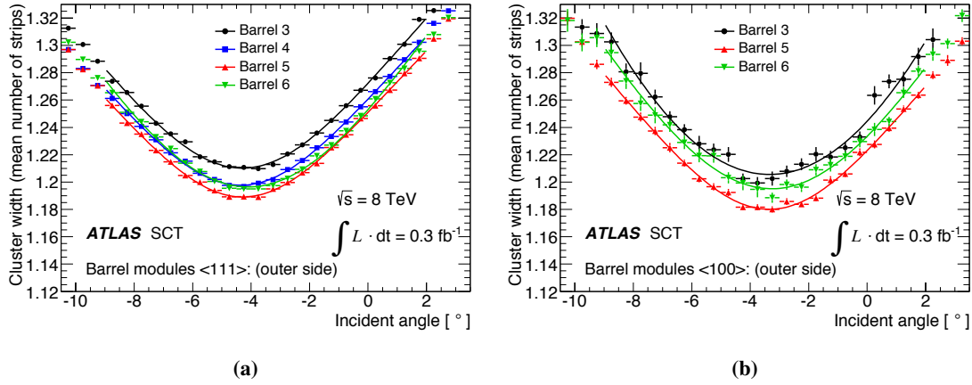
Figure 21. Cluster-size dependence on the particle incident angle for each SCT barrel for (a) \langle 111 \rangle sensors and (b) \langle 100 \rangle sensors. The displacement of the minimum from zero is a measurement of the Lorentz angle \theta_L .
