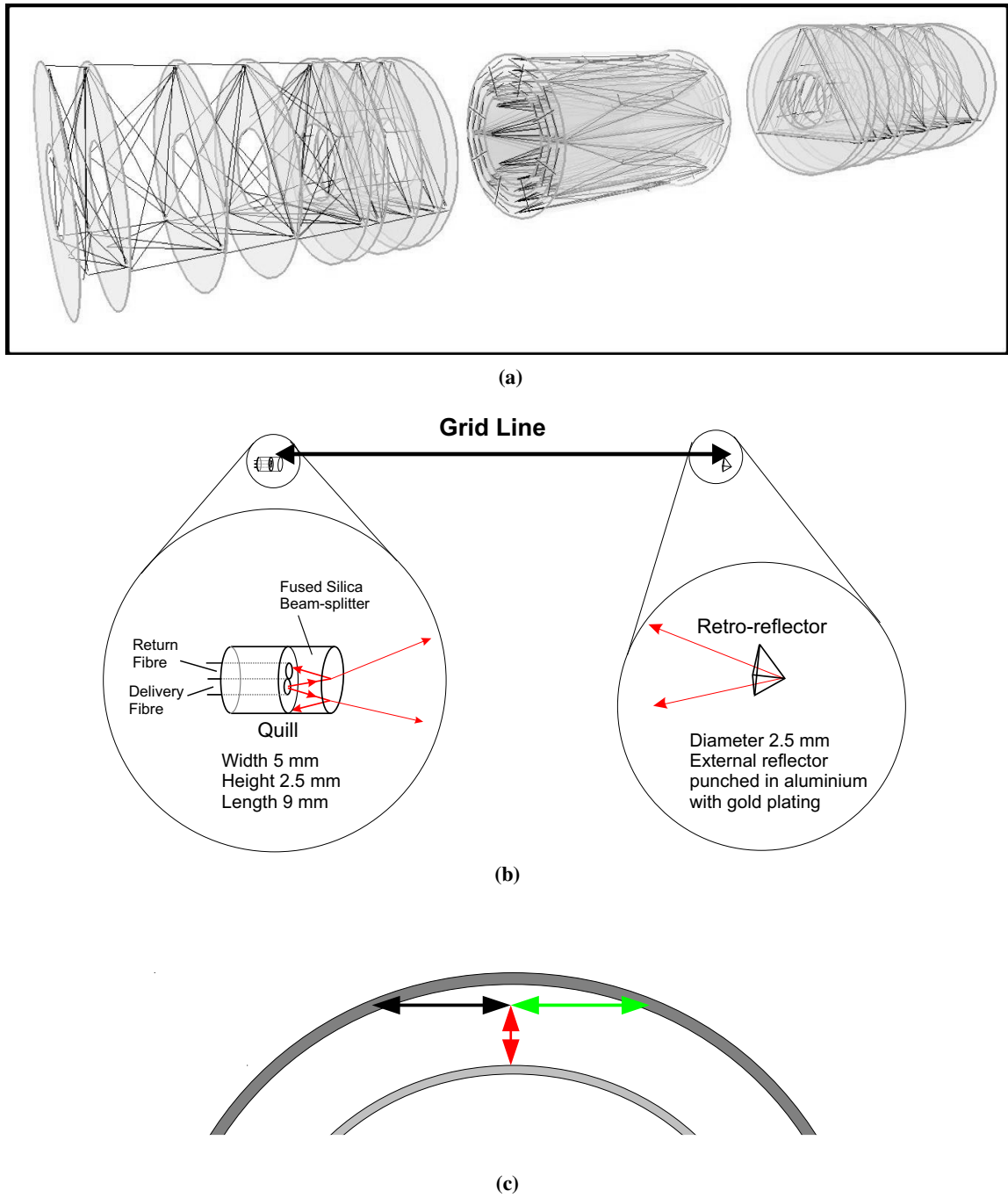
Figure 4. (a) The FSI grid layout across the SCT volume. (b) The grid-line interferometer design for the FSI system. (c) The arrangement of each group of three grid-line interferometers on the barrel flange. The colours used here for each line in the assembly are replicated in section 6.3.
