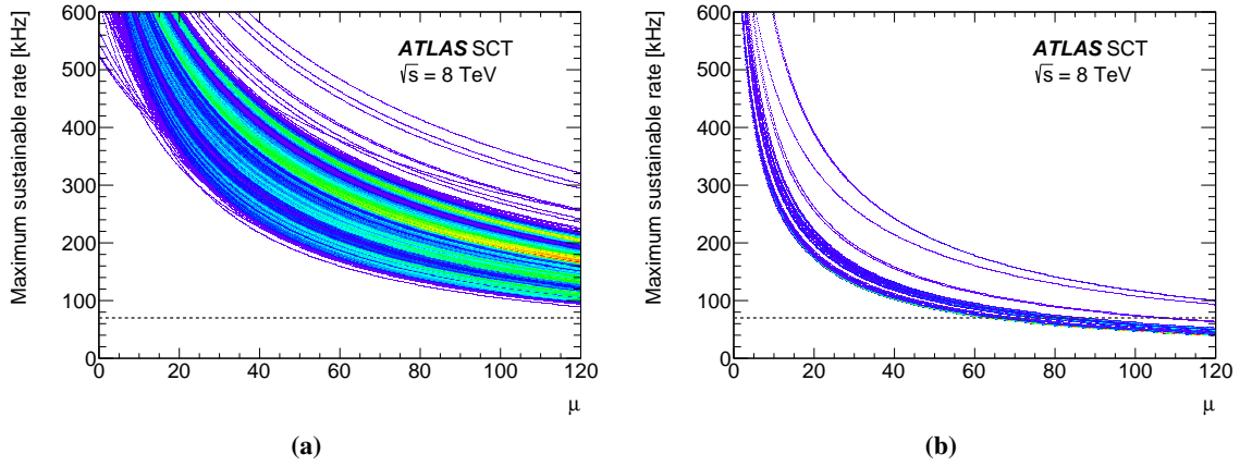
Figure 12. Maximum sustainable level-1 trigger rate for the transfer of data from (a) front-end chip to ROD and (b) ROD to ATLAS DAQ chain, as a function of the mean number of interactions per bunch crossing, \mu . Values are calculated from measured event sizes in pp interactions at \sqrt{s} = 8 TeV assuming 90% of the available data-link bandwidth is used. Each link is shown as a separate curve. Increasing numbers of superimposed curves are indicated by changes of colour from blue through green and yellow to red. The dashed lines indicate the typical 2012 trigger rate of 70 kHz.
