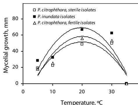
Figure 2. Growth temperature curves obtained with sterile and fertile isolates of Phytophthora citrophthora and isolates of P. inundata obtained from citrus trees in Chile. Polynomial equations for P. citrophthora were y = -0.18x^2 + 7.23x - 20.50 ( R^2 = 0.68 ) and y = -0.22x^2 + 8.58x - 27.49 ( R^2 = 0.75 ) for sterile and fertile isolates, respectively. Polynomial equation for isolates of P. inundata was y = -0.24x^2 + 9.44x - 23.20 ( R^2 = 0.72 ).
