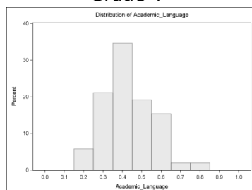
Figure 1: Series of histograms displaying the distribution of total CALS-I scores within grade Grade 4
