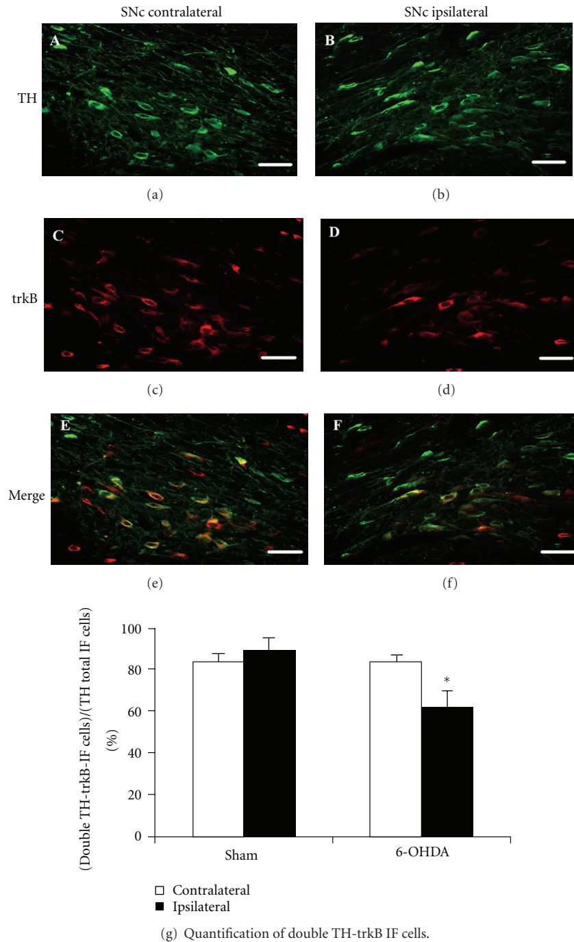
FIGURE 6: A decrease in the percentage of double labeling for TH and trkB in SNc is detected 7 days after unilateral 6-OHDA intrastratial injections. Photomicrographs show TH-IF cells (a), (b) and trkB-IF cells (c), (d) in rat SNc, 7 days after unilateral 6-OHDA intrastratial injection. (e) Merge of (a) and (c); (f) merge of (b) and (d). (a), (c), and (d) correspond to contralateral SNc while (b), (d), and (f) to ipsilateral SNc. (a)–(f) scale bar = 50 μm. SNc: substantia nigra pars compacta. (g) Quantification of cells that coexpress TH and trkB in the ipsilateral SNc compared to their contralateral side, 7 days after unilateral 6-OHDA or ascorbic acid (sham) intrastratial injections to rats. The results were expressed as the percentage of cells that coexpress TH and trkB over the number of total TH-IF cells. Number of cells with TH-IF signals and double TH-trkB-IF signals in contralateral SNc after ascorbate injection was 365.1 \pm 39.7 and 309.5 \pm 39.7 cells/mm 2 , respectively. In the case of 6-OHDA-treated rats, number of cells with TH-IF signals and double TH-trkB-IF signals in contralateral SNc was 333.3 \pm 23.8 and 277.7 \pm 7.9 cells/mm 2 , respectively. n = 4 rats for each experimental condition. The different experimental groups were compared by a Kruskal-Wallis nonparametric ANOVA, followed by a U -test. * P < 0.05 compared with sham-treated rats.
