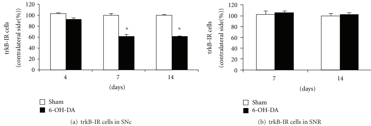
FIGURE 3: Unilateral 6-OHDA intrastratial injection results in a significant decrease in the number of trkB-IR cells in ipsilateral SNc at 7 and 14 days after the injection. (a) Percentage of trkB-IR cells in rat ipsilateral SNc compared to the contralateral side after unilateral 6-OHDA (black columns) or ascorbic acid (sham, white columns) intrastratial injections. Number of cells with trkB-IR signals in contralateral SNc of ascorbate-injected rats per area unit per slice was 507.9 \pm 7.9 , 365.1 \pm 15.9 , and 412.7 \pm 10.6 cells/mm 2 , at 4, 7, and 14 days after injections, respectively. In the case of 6-OHDA-treated rats, number of cells with trkB-IR signals in contralateral SNc was 484.1 \pm 15.9 , 381.0 \pm 31.7 and 404.7 \pm 15.9 cells/mm 2 , at 4, 7, and 14 days after 6-OHDA injections, respectively. (b) Percentage of trkB-IR cells in the ipsilateral SNR compared to the contralateral side, at 7 and 14 days after unilateral intrastratial injections of 6-OHDA (black columns) or ascorbic acid (sham, white columns). Number of cells with trkB-IR signals in contralateral SNR of ascorbate-treated rats was 117.9 \pm 5.1 and 143.6 \pm 5.1 cells/mm 2 , at 7 and 14 days after injections, respectively. In the case of 6-OHDA-treated rats, the number of cells with trkB-IR signals in contralateral SNR amounted to 117.9 \pm 5.1 and 148.7 \pm 10.3 cells/mm 2 , at 7 and 14 days after toxin injections, respectively. n = 6 rats under each experimental condition. The different experimental groups were compared by a Kruskal-Wallis nonparametric ANOVA, followed by a U-test. * P < 0.05 compared with sham-treated rats.
