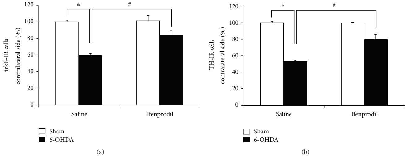
FIGURE 7: Ifenprodil, an antagonist of NR2B containing NMDA receptors, prevents the decrease in trkB-IR and TH-IR cells occurring in SNc 14 days after 6-OHDA intrastratial injection. Positive cells for trkB and TH immunostaining in SNc were counted in coronal midbrain slices of treated rats as described in Section 2. Four groups of rats in each case (a) and (b) were pretreated with saline solution or Ifenprodil (5 mg/kg, i.p.), 1 day before and 3, 5, and 7 days after unilateral 6-OHDA (black columns) or ascorbic acid (sham, white columns) intrastratial administration. The IHC studies were performed 14 days after 6-OHDA or ascorbic acid injections. Results were expressed as a percentage of trkB-IR cells (a) or TH-IR cells (b) in the ipsilateral SNc compared with the contralateral side. (a) Number of cells with trkB-IR signals in sample areas per slice from contralateral SNc was equal to 365.1 \pm 15.9 , 381.0 \pm 31.7 , 412.7 \pm 10.6 , and 404.7 \pm 15.9 cells/mm 2 in sham-saline, 6-OHDA-saline, sham-Ifenprodil, and 6-OHDA-Ifenprodil rats, respectively. (b) Number of TH-IR cells in sample areas per slice from contralateral SNc was equal to 404.8 \pm 23.8 , 357.1 \pm 29.8 , 386.9 \pm 11.9 , and 369.0 \pm 6.0 cells/mm 2 in sham-saline, 6-OHDA-saline, sham-Ifenprodil, and 6-OHDA-Ifenprodil rats, respectively. The different experimental groups were compared by a Kruskal-Wallis nonparametric ANOVA, followed by a U -test. * P < 0.05, when comparing saline-6-OHDA versus saline-sham rats. # P < 0.05 when comparing saline-6-OHDA versus Ifenprodil-6OHDA rats. n = 3 rats under each experimental condition.
