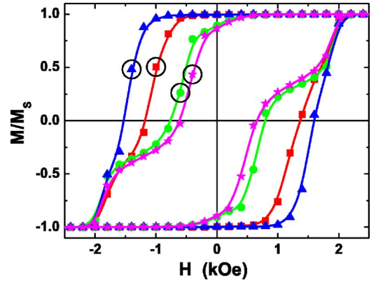
FIG. 6. (Color online) Hysteresis loops of a magnetic dot of D=65 nm and H=20 nm for four different types of anisotropy: easy-axis (triangles), cubic (squares), easy-plane (circles), and no anisotropy (stars). Points at which the vortex first enters the dot are circled in black.
