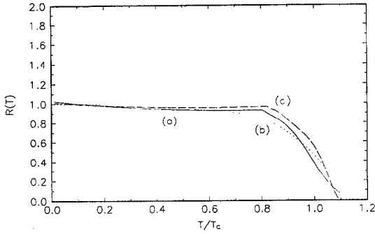
Fig. 1. The ratios f_\pi^2(T)/f_\pi^2(0) , Solid curve (a); \langle \bar{q}q \rangle_T / \langle \bar{q}q \rangle , dotted curve (b), both from [3]; and s_0(T)/s_0(0) , dashed curve (c), from the FESR Eq. (10).
