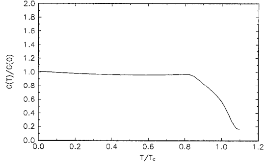
Fig. 2. The ratio of the GMOR relation, Eq. (14).
