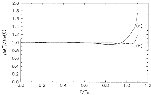
Fig. 3. The ratio \mu_\pi(T)/\mu_\pi(0) obtained by solving the FESR Eq. (12), curve (a), and Eq. (13), curve (b). In both cases, f_\pi(T) and \langle \bar{q}q \rangle_T from [3] were used as input.
