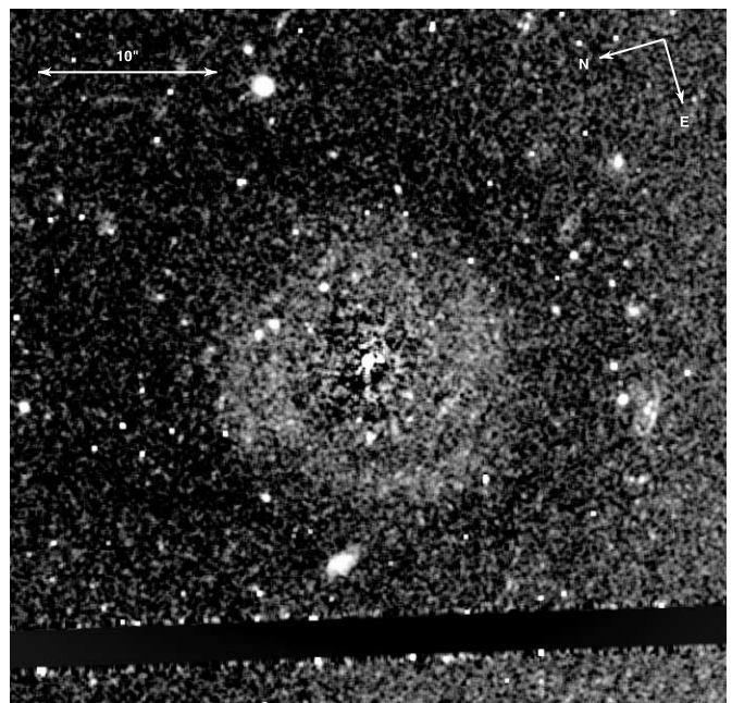
FIG. 110.—Residual images of VCC 1695 ( left ) and VCC 1199 ( right ), obtained by subtracting the best-fitting isophotal model from the g -band images. Both galaxies appear to display a spiral pattern. Each image is 40'' on the side.
