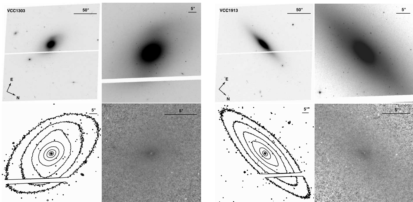
FIG. 21.— Left : VCC 1303 (=NGC 4483, Hubble type SB 0 (5)). Right : VCC 1913 (=NGC 4623, Hubble type E7). See Fig. 1 for details.
