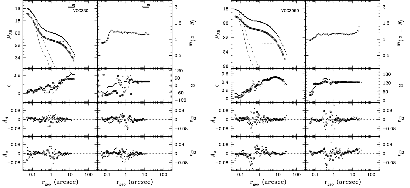
FIG. 93.— Left: VCC 230 (=IC 3101, Hubble type dE4;N). Right: VCC 2050 (=IC 3779, Hubble type dE5;N). See Fig. 51 for details.
