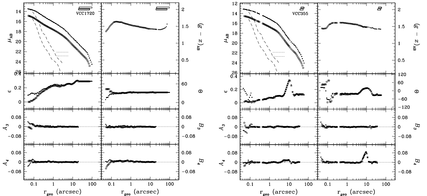
FIG. 64.—Left: VCC 1720 (=NGC 4578, Hubble type S0 1/2 (4)). Right: VCC 355 (=NGC 4262, Hubble type SB0 2/3 ). See Fig. 51 for details.
