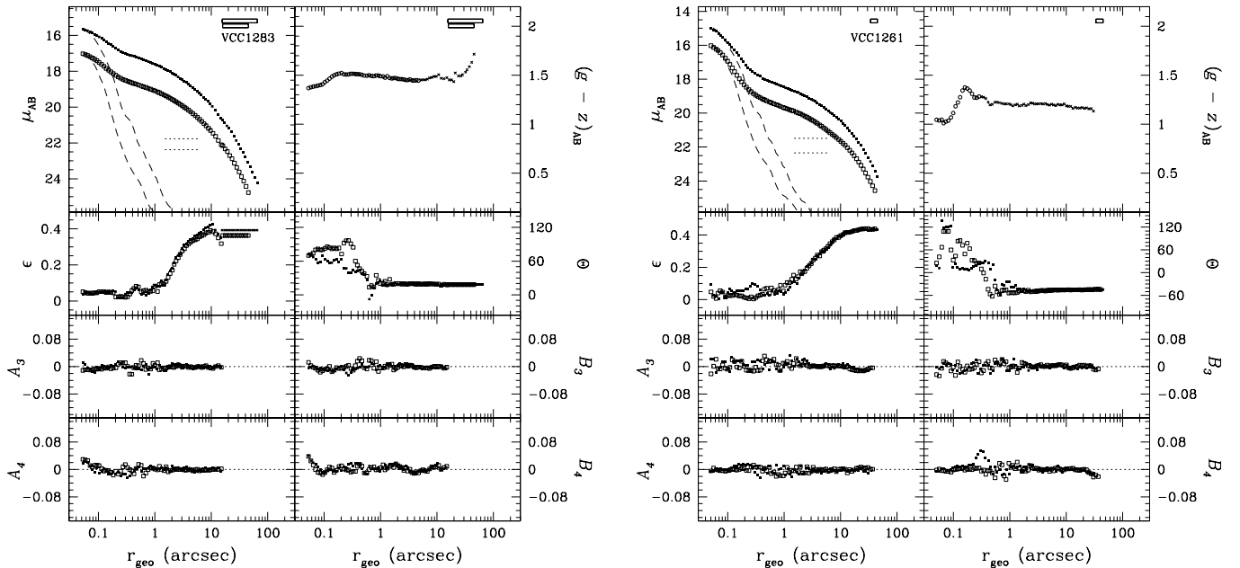
FIG. 74.— Left: VCC 1283 (=NGC 4479, Hubble type SB0 2 (2)). Right: VCC 1261 (=NGC 4482, Hubble type d:E5,N). See Fig. 51 for details.
