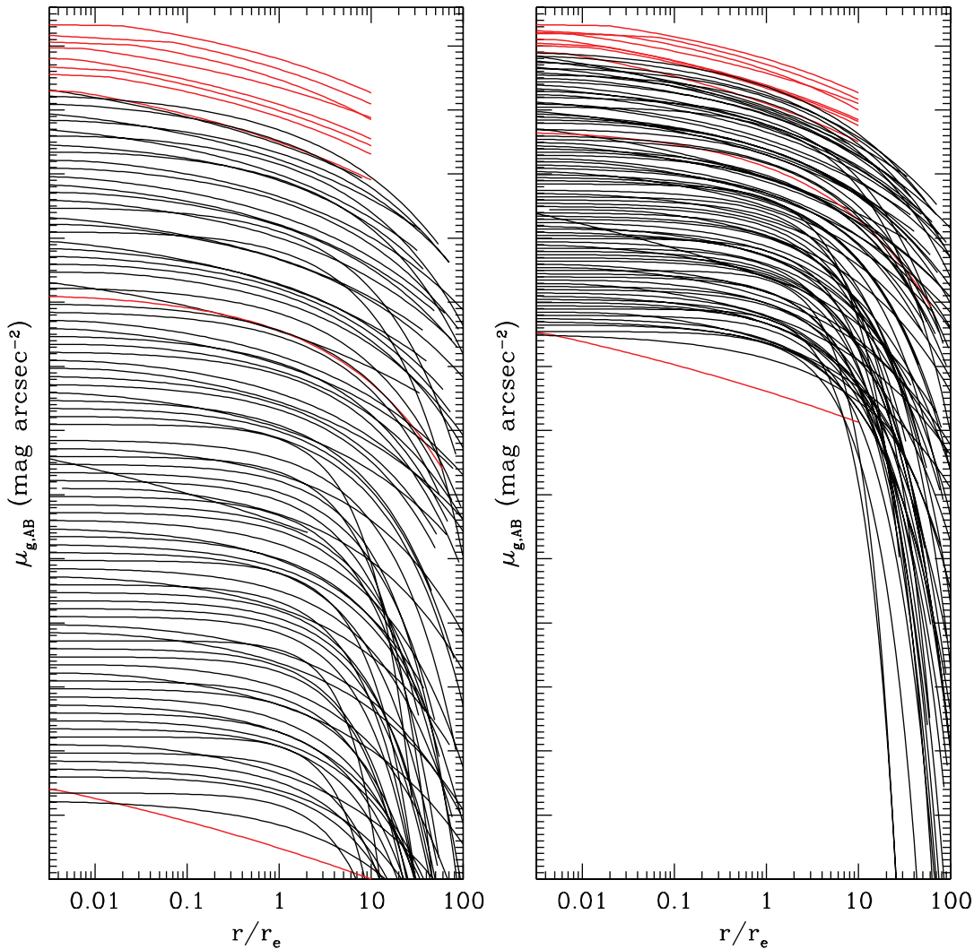
FIG. 112.—A compilation of the best-fit models for the g -band surface brightness profiles of all ACSVCS galaxies. The models exclude a nuclear component when present and are shown before convolution by the ACS/WFC PSF. For each galaxy, the abscissa shows the isophotal radius normalized to the effective radius r_e , derived from the best fit. Along the ordinate, galaxies are ordered according to their total B -band magnitudes, with the brightest galaxy (VCC 1226) plotted as having the largest central surface brightness, and every other galaxy plotted as having central surface brightness shifted downward, by a constant amount, relative to that of VCC 1226. Each small tick on the ordinate corresponds to 1 \text{ mag arcsec}^{-2} . The two panels differ only in the range of surface brightness shown: to the right, the scale is shown to highlight difference in the innermost region. In both panels, galaxies best fit by a core-Sérsic profile are shown in red.
