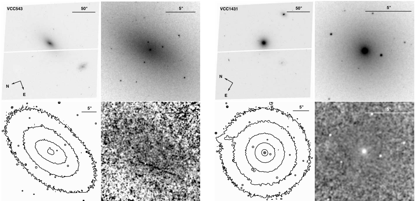
FIG. 32.— Left : VCC 543 (=UGC 7436, Hubble type dE5). Right : VCC 1431 (=IC 3470, Hubble type dE0,N). See Fig. 1 for details.
