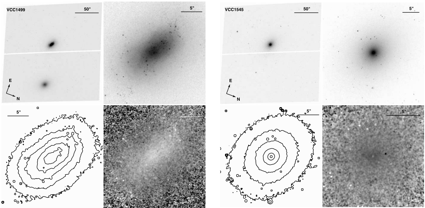
FIG. 39.— Left : VCC 1499 (=IC 3492, Hubble type E3 pec or S0). Right : VCC 1545 (=IC 3509, Hubble type E4). See Fig. 1 for details.
