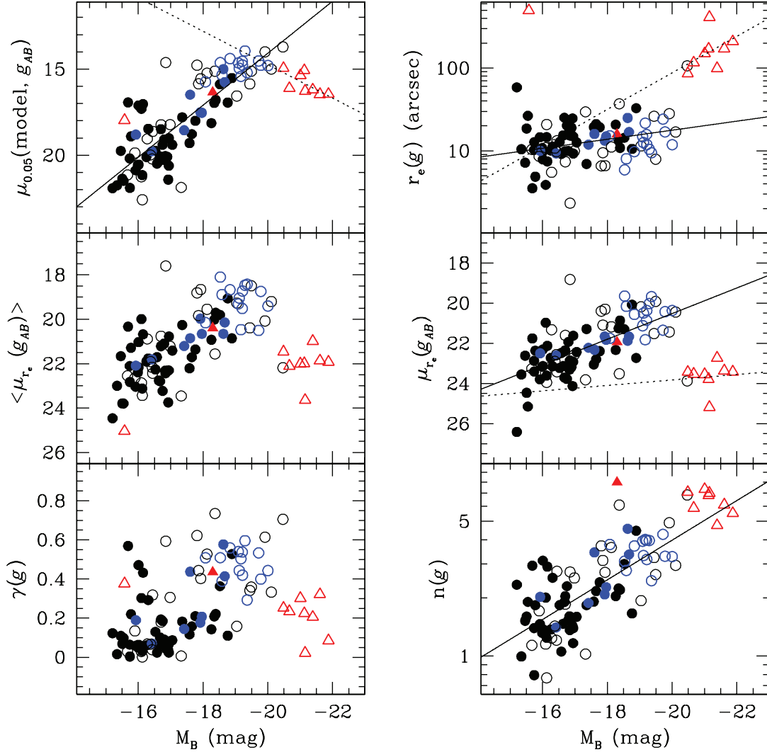
FIG. 117.— Correlation of parameters characterizing the inner (on the left) and outer (on the right) surface brightness profile and the total B -band magnitude of the host galaxies. On the left panels, from top to bottom, are shown the surface brightness measured from the best-fitting model at 0''.049 , prior to PSF convolution and excluding a nuclear component, if present; the average surface brightness within one effective radius r_e , in \text{mag arcsec}^{-2} ; and the slope \gamma of the inner profile at r = 0''.1 , measured prior to PSF convolution (following eq. [16] in the case of profiles best fitted by a Sérsic model). On the right panels are shown the effective radius r_e ; the surface brightness at r_e , in \text{mag arcsec}^{-2} ; and the Sérsic index n characterizing the shape of the outer profile. Galaxies are color-coded as in the legend of Fig. 115, blue points refer to galaxies with multiple morphological components.
