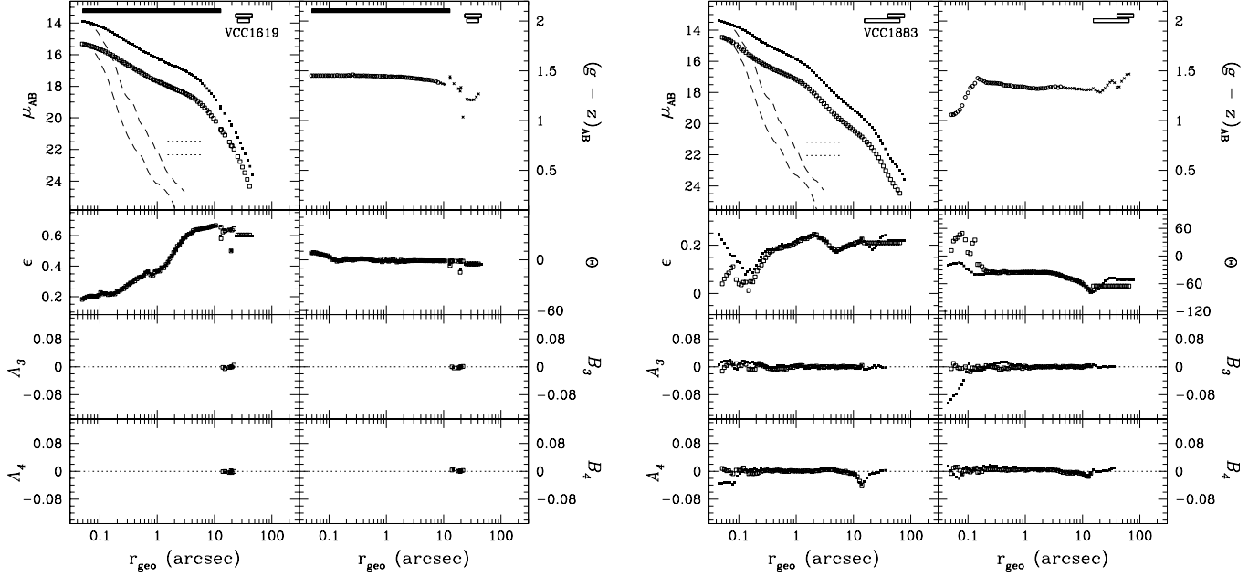
FIG. 65.— Left: VCC 1619 (=NGC 4550, Hubble type E7/S0 1 (7)). Right: VCC 1883 (=NGC 4612, Hubble type RSB0 1/2 ). See Fig. 51 for details.
