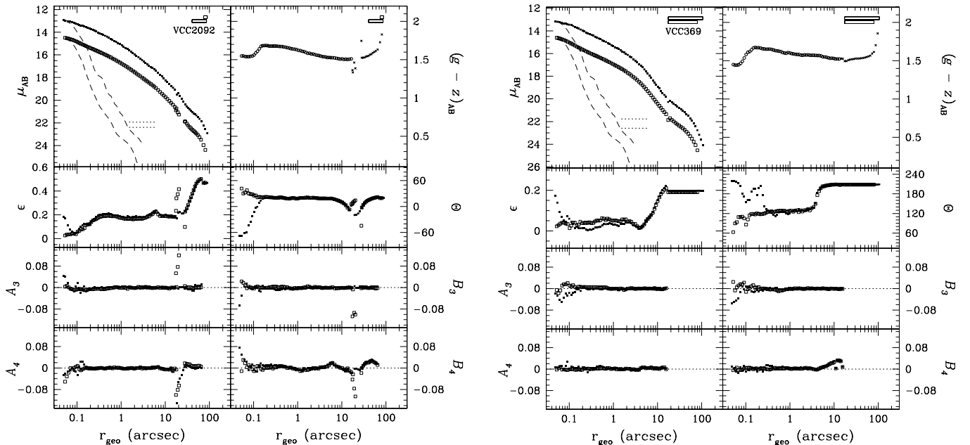
FIG. 58.— Left : VCC 2092 (=NGC 4754, Hubble type SB0 1 (5)). Right : VCC 369 (=NGC 4267, Hubble type SB0 1 ). See Fig. 51 for details.
