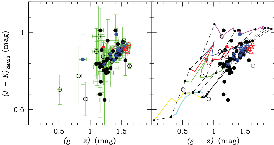
FIG. 124.— g - z vs. J - K color-color diagrams. J - and K -band magnitudes are from the 2MASS database. Galaxies are coded as in Fig. 123, as are the stellar population synthesis models. All magnitudes have been extinction corrected.
