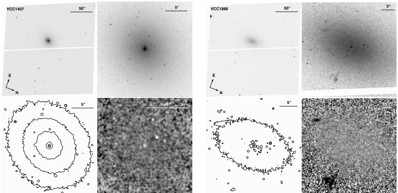
FIG. 46.— Left : VCC 1407 (=IC 3461, Hubble type dE2,N). Right : VCC 1886 (Hubble type dE5,N). See Fig. 1 for details.
