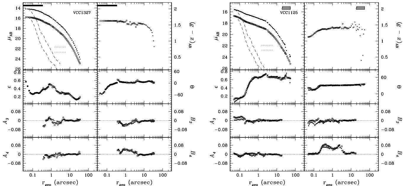
FIG. 72.— Left: VCC 1327 (=NGC 4486A, Hubble type E2). Right: VCC 1125 (=NGC 4452, Hubble type S0 1 (9)). See Fig. 51 for details.
