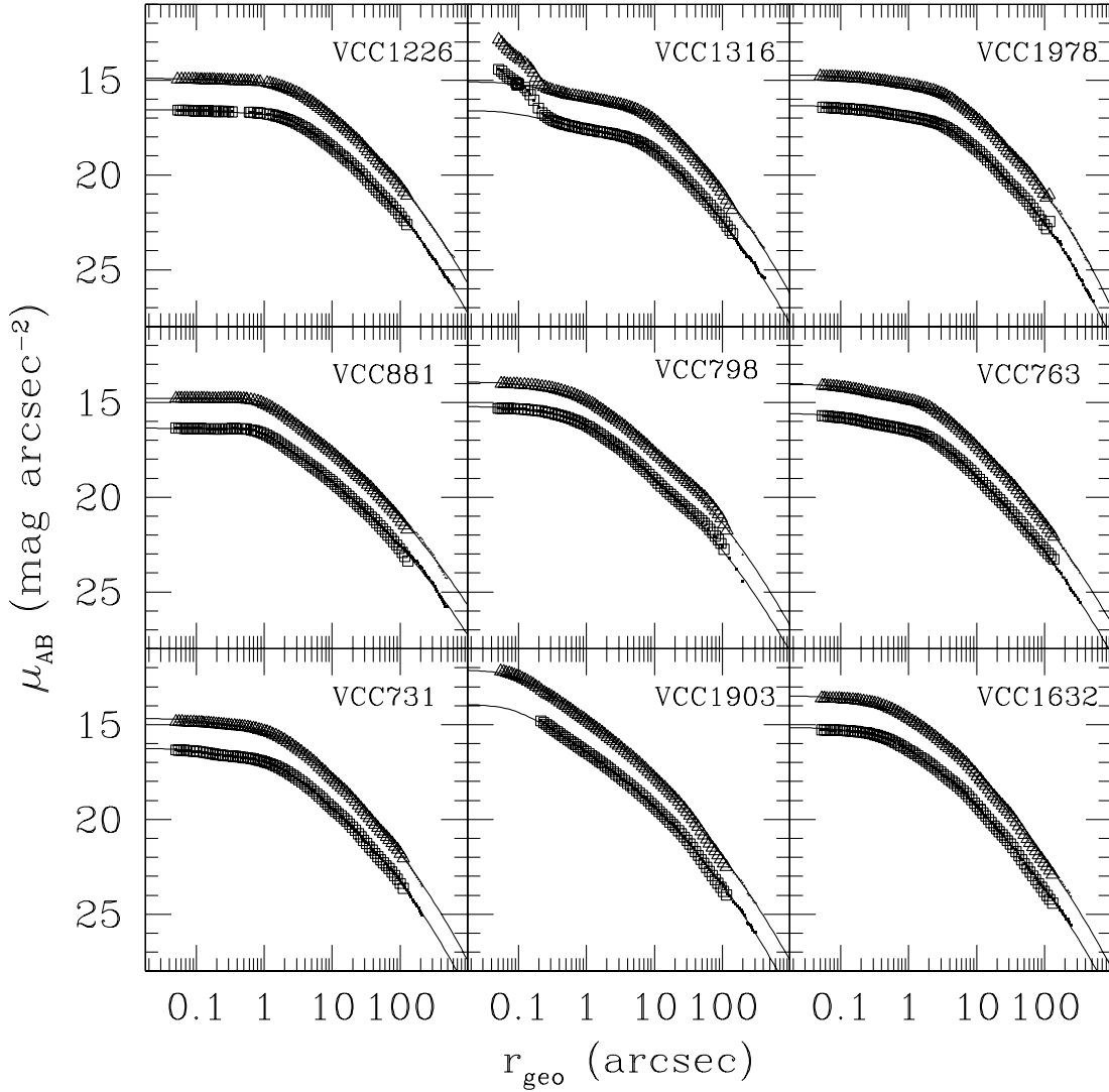
FIG. 102.— Composite surface brightness profiles, obtained by combining the ACSVCS g - and z -band profiles (shown as open symbols) with ground-based B -band profiles drawn from the literature, and plotted as a function of the geometric mean radius. The solid curve represents the best-fit core-Sérsic model to the final composite profile (shown as solid symbols). For each galaxy, the brighter of the two profiles is measured in the z band.
