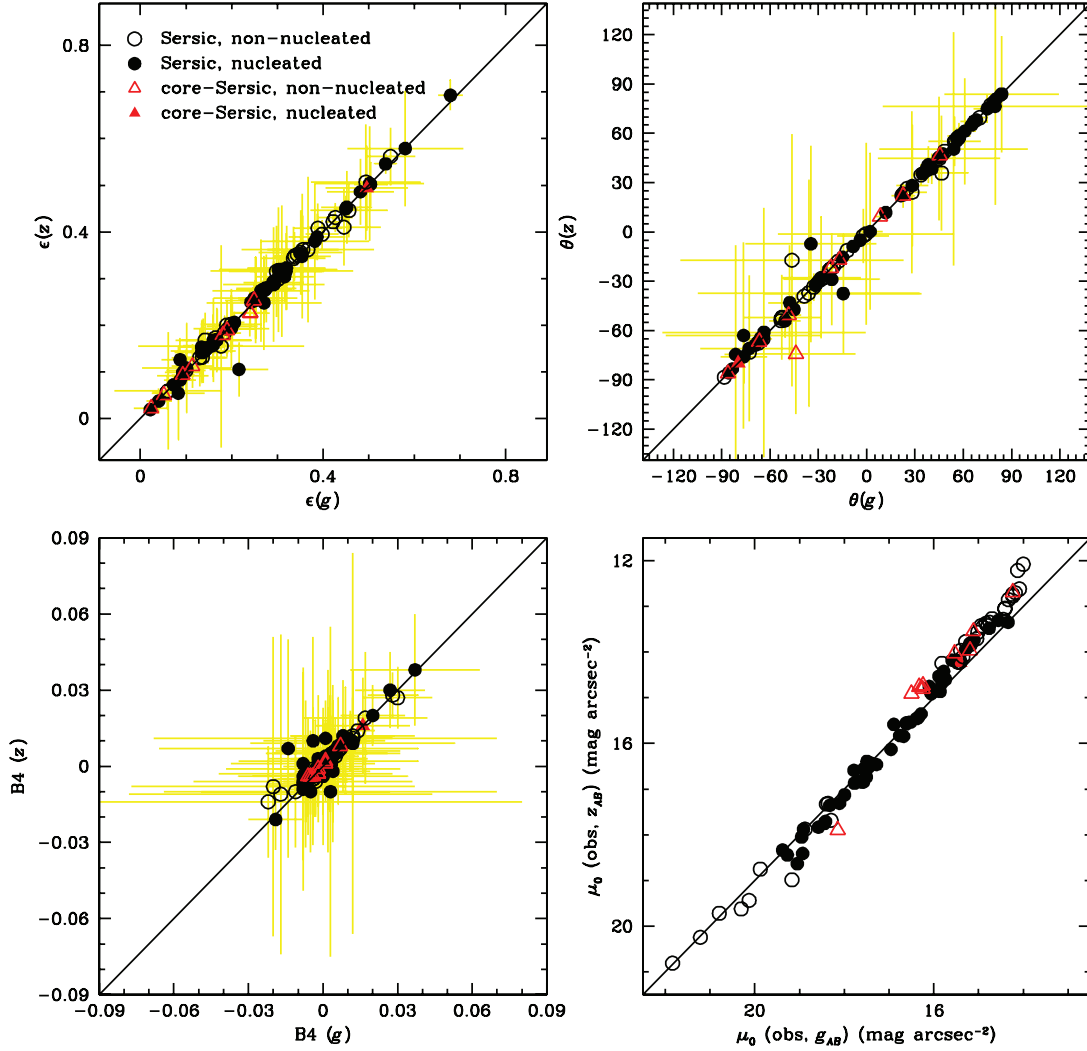
FIG. 101.— Comparison of the mean ellipticity, \epsilon , position angle, \theta , B4 coefficients, and extinction-corrected central surface brightness, \mu_0 , measured in the g and z bands. The mean values are calculated between 1'' and one effective radius, excluding regions affected by dust or nuclei. Standard deviations from the mean values are plotted in yellow to avoid overcrowding the plot—such standard deviations are overestimates of the intrinsic errors in the mean, since they are affected by real radial variation in \epsilon , \theta , and B4. Filled and open symbols represent nucleated and non-nucleated galaxies, respectively. Galaxies best fitted by a Sérsic profile are shown in black; galaxies best fitted by a core-Sérsic profile are shown in red (see § 3.3).
