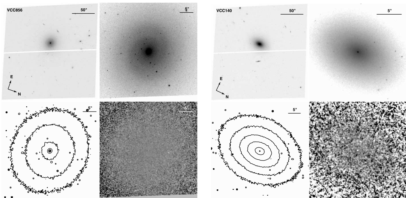
FIG. 29.— Left : VCC 856 (=IC 3328, Hubble type dE1,N). Right : VCC 140 (=IC 3065, Hubble type S0 1/2 (4)). See Fig. 1 for details.
