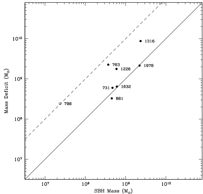
FIG. 119.—Core “mass deficit,” defined as the difference between the mass enclosed within the break radius by the Sérsic model that best fits the outer surface brightness profile and the best-fit core-Sérsic model, plotted against the mass estimated for the nuclear SBH (see text for details). The solid and dashed lines are plotted for a mass deficit equal to, and 10 times larger than, the SBH mass. VCC 798 (NGC 4382), shown by the open circle, is likely to host a large-scale stellar disk.
