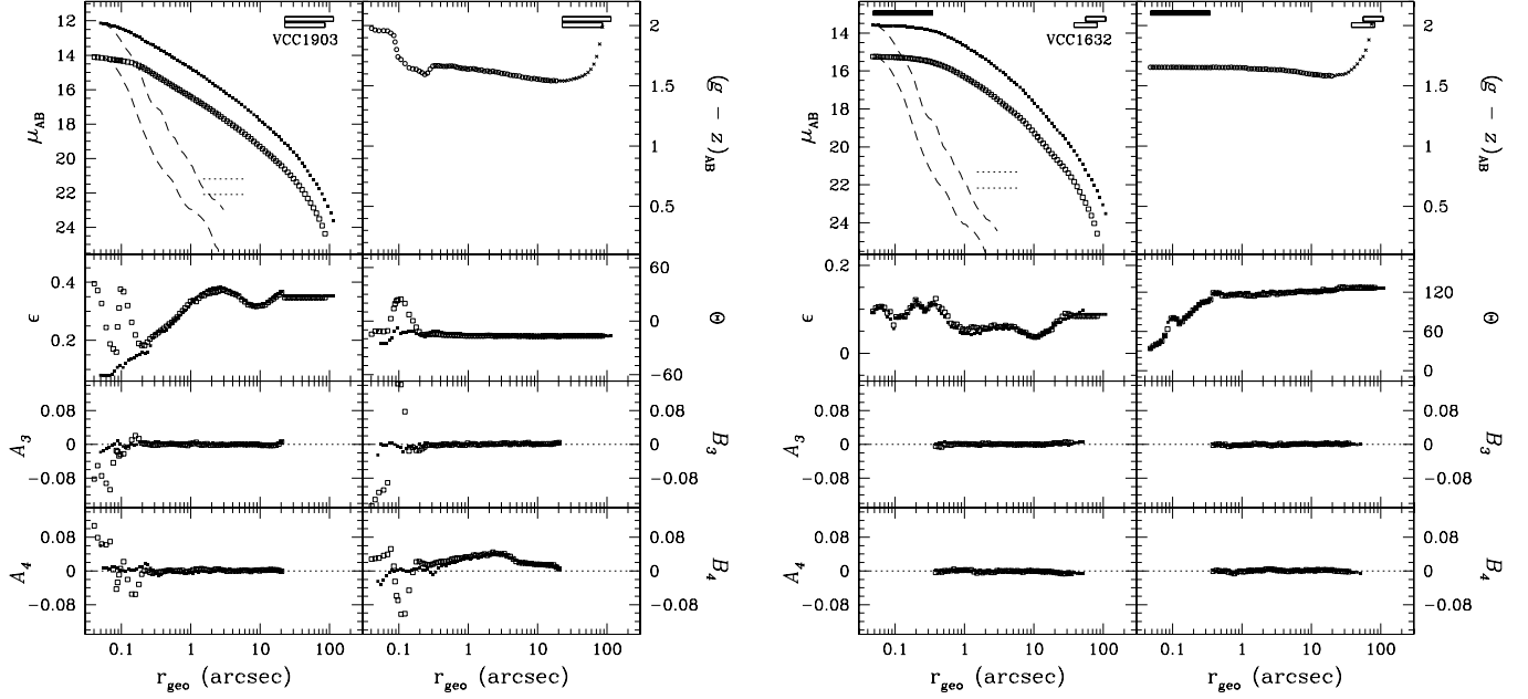
FIG. 55.— Left : VCC 1903 (=M59, NGC 4621, Hubble type E4). Right : VCC 1632 (=M89, NGC 4552, Hubble type S0 1 (0)). See Fig. 51 for details.
