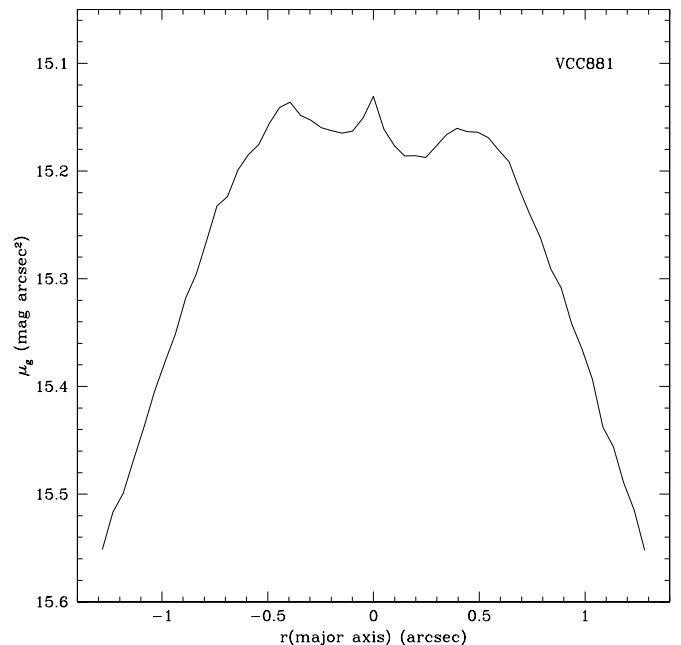
FIG. 108.—A cut through the g -band photometric major axis of VCC 881 (NGC 4406), showing the decrease in the surface brightness profile in the inner 0''.4 .
