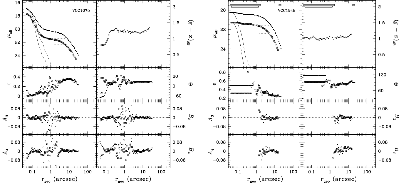
FIG. 91.—Left: VCC 1075 (=IC 3383, Hubble type dE4,N). Right: VCC 1948 (Hubble type dE3). See Fig. 51 for details.
