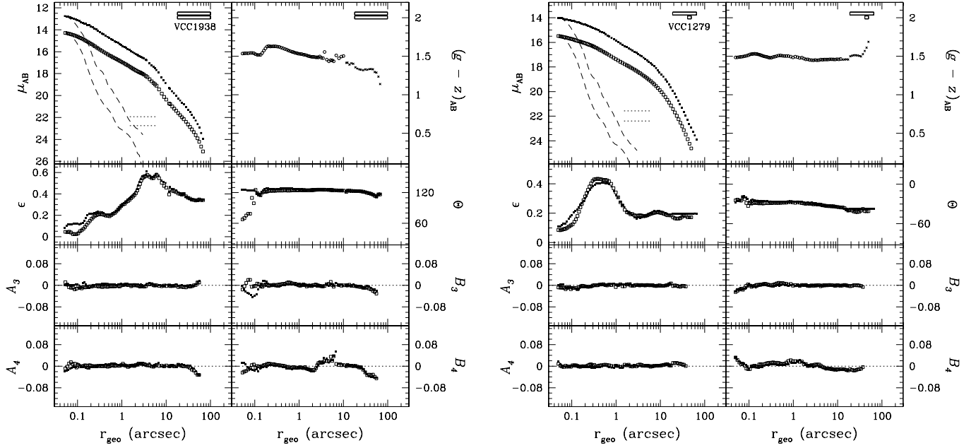
FIG. 63.—Left: VCC 1938 (=NGC 4638, Hubble type S0 1 (7)). Right: VCC 1279 (=NGC 4478, Hubble type E2). See Fig. 51 for details.
