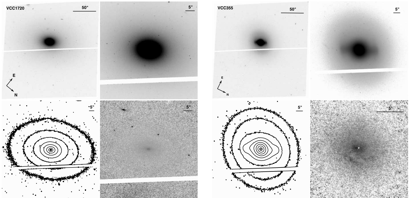
FIG. 14.— Left : VCC 1720 (=NGC 4578, Hubble type S0_{1/2}(4) ). Right : VCC 355 (=NGC 4262, Hubble type SB0_{2/3} ). See Fig. 1 for details.
