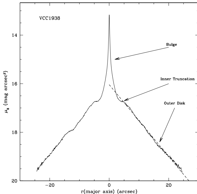
FIG. 105.— Left : Cut through the g -band photometric major axis of VCC 1938 (NGC 4638), clearly showing the inner truncation of the outer exponential disk. Right : Residual map, obtained by subtracting the best-fitting isophotal model from the g -band image. To avoid overcrowding the image, labels are superimposed only to the northwest side of the disk. The disk shows as a positive residual in the map.
