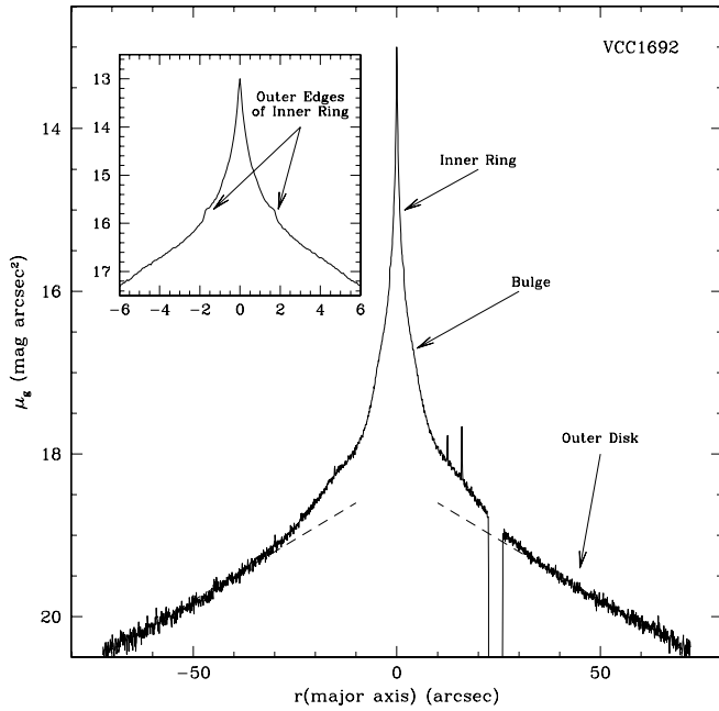
FIG. 104.—A cut through the g -band photometric major axis of VCC 1692 (NGC 4570), highlighting the several morphological components. As shown by the dashed line, the outer profile, dominated by a thin stellar disk, is roughly exponential. The bulge contribution is visible in the inner \sim 20'' . The innermost 1''.8 are dominated by the nuclear ring, the outer boundary of which are clearly visible in the expanded view shown in the inset.
