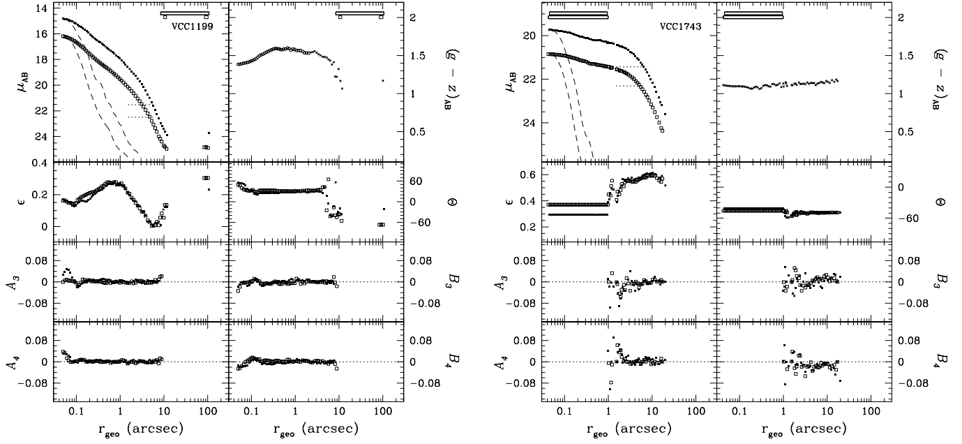
FIG. 97.— Left: VCC 1199 (Hubble type E2). Right: VCC 1743 (=IC 3602, Hubble type dE6). See Fig. 51 for details.
