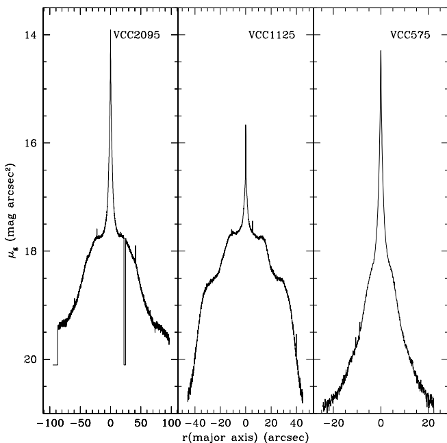
FIG. 107.—Cuts through the g -band photometric major axes of VCC 2095 (NGC 4762), VCC 1125 (NGC 4452), and VCC 575 (NGC 4318).
