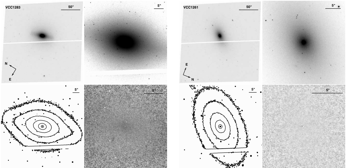
FIG. 24.— Left : VCC 1283 (=NGC 4479, Hubble type SB0 2 (2)). Right : VCC 1261 (=NGC 4482, Hubble type d:E5,N). See Fig. 1 for details.
