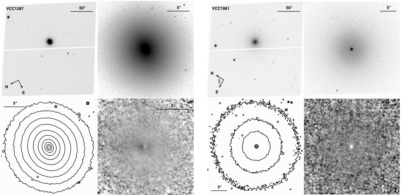
FIG. 31.— Left : VCC 1297 (=NGC 4486B, Hubble type E1). Right : VCC 1861 (=IC 3652, Hubble type dE0,N). See Fig. 1 for details.
