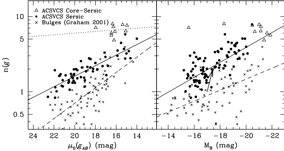
FIG. 120.— Left : The Sérsic index n , plotted against the surface brightness estimated from the best-fitting model at 0''.049 , prior to PSF convolution. Right : n , plotted against the total, extinction-corrected absolute B -band magnitude of the host galaxy (from the RC3). The ACSVCS galaxies are shown as solid circles and open triangles depending on whether the surface brightness profile is best fitted by a Sérsic or core-Sérsic model, respectively. Crosses represent bulges from Graham (2001); B -band central surface brightnesses from this paper have been converted to g band by assuming g - B \sim 0.55 (Fukugita et al. 1995), in addition the bulge data have been extinction-corrected and total magnitudes have been rescaled to H_0 = 72 \text{ km s}^{-1} \text{ Mpc}^{-1} . The solid line represents the best least-squares fit to the “Sérsic” galaxies (filled circles), the dotted line shows the best least-squares fit to the “core-Sérsic” galaxies, and the dashed line shows the best fit to the bulges. The arrow in the bottom right panel shows the change in n and M_B undergone by an exponential ( n = 1 ) bulge after merging with a satellite of half its mass, according to N -body simulations by Eliche-Moral et al. (2005).
