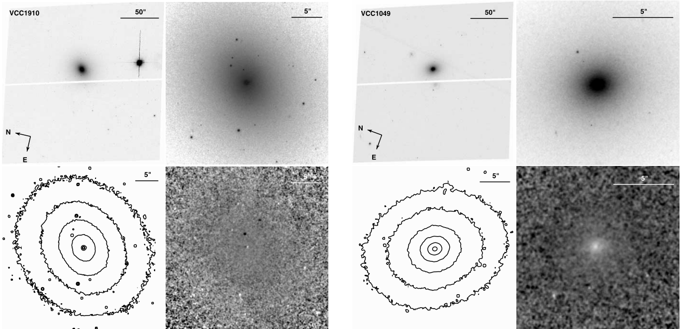
FIG. 28.— Left : VCC 1910 (=IC 809, Hubble type dE1,N). Right : VCC 1049 (=UGC 7580, Hubble type S0(4)). See Fig. 1 for details.
