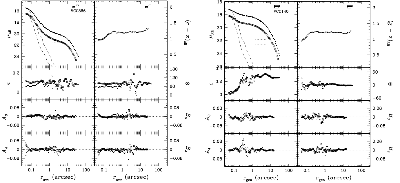
FIG. 79.— Left : VCC 856 (=IC 3328, Hubble type dE1,N). Right : VCC 140 (=IC 3065, Hubble type S0 1/2 (4)). See Fig. 51 for details.
