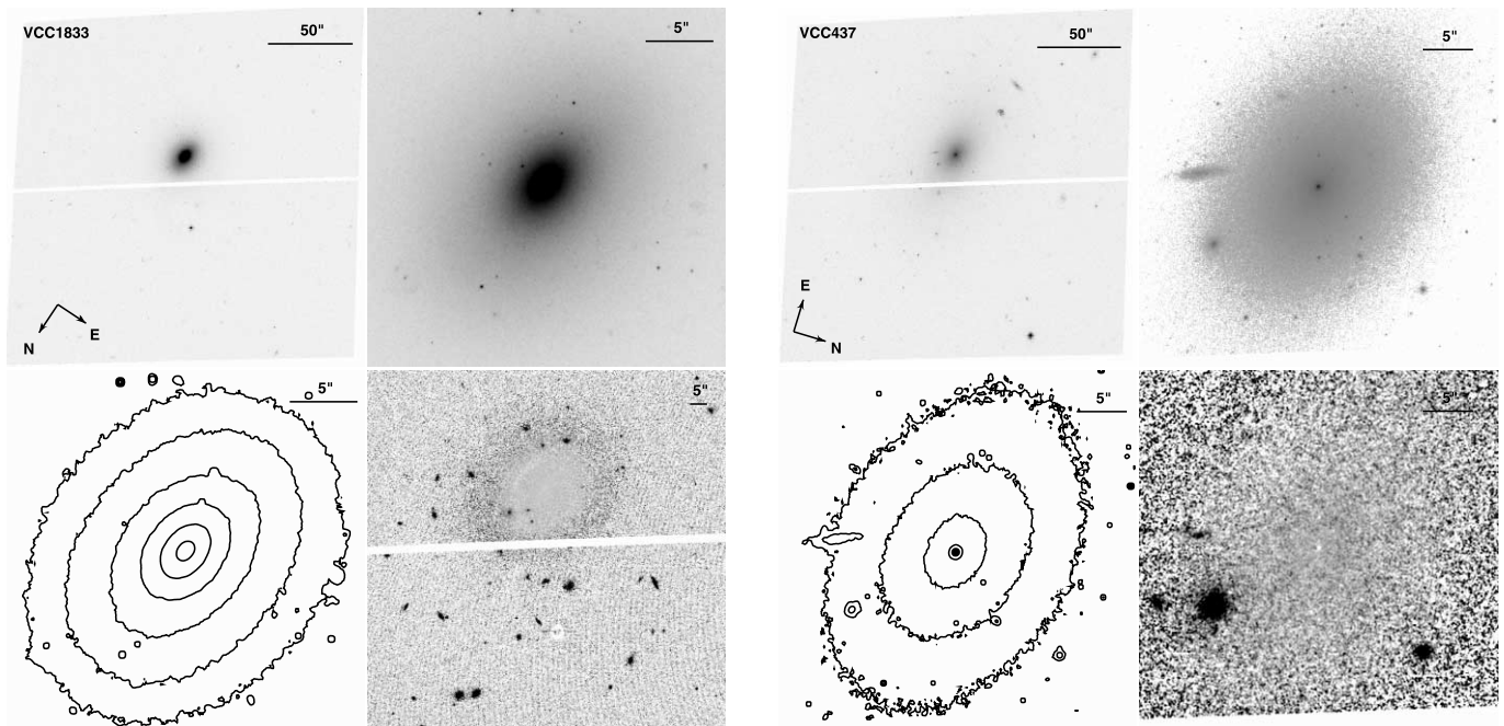
FIG. 34.— Left : VCC 1833 (Hubble type S0 1 (6)). Right : VCC 437 (=UGC 7399A, Hubble type dE5,N). See Fig. 1 for details.
