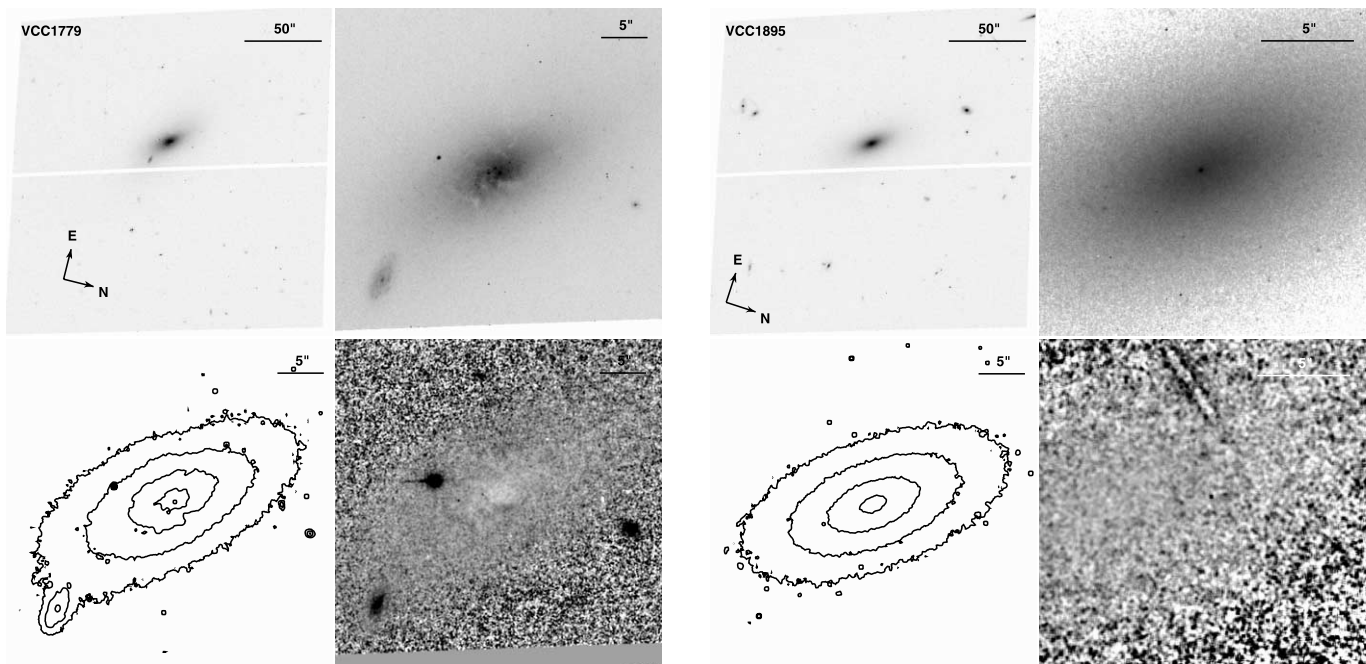
FIG. 38.— Left: VCC 1779 (=IC 3612, Hubble type dS0(6):). Right: VCC 1895 (=UGC 7854, Hubble type d:E6). See Fig. 1 for details.
