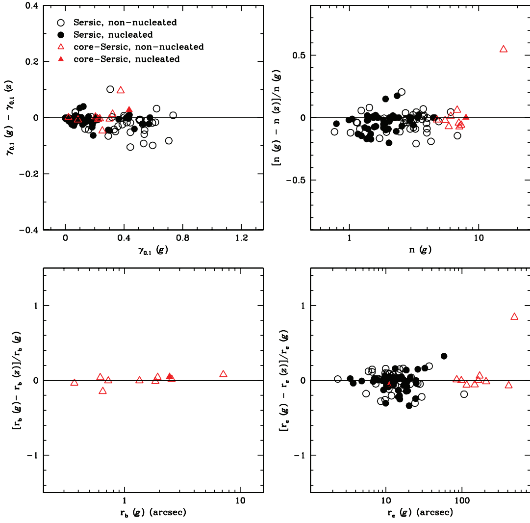
FIG. 114.— Comparison of \gamma , n , break and effective radii ( r_b and r_e ) for the best fits to the surface brightness profiles in the g and z bands. Galaxies are color-coded as in Fig. 101. In the case of galaxies best fitted by a Sérsic profile, the logarithmic slope \gamma is calculated at 0''.1 from the center and is uniquely defined by n and r_e (see eq. [16]).
