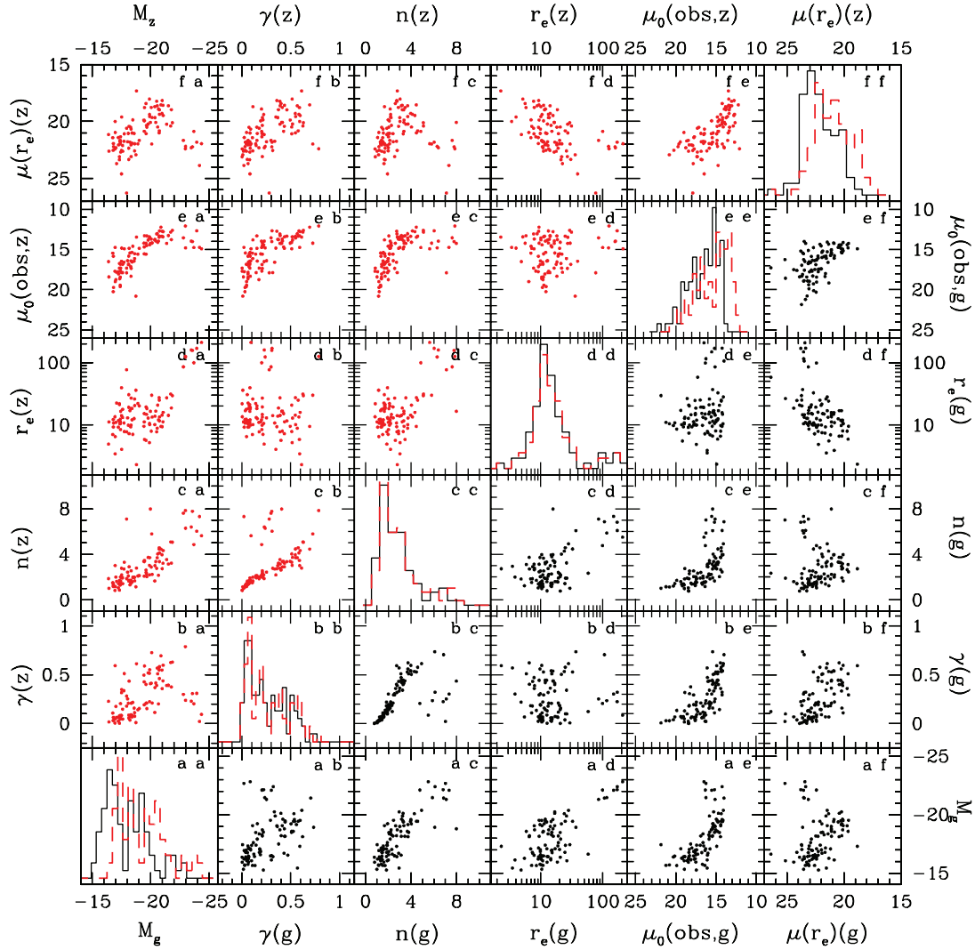
FIG. 116.— Correlations between fit parameters: total absolute magnitude from the model profile, integrated to infinity and extinction corrected; inner slope \gamma (in the case of galaxies best fitted by a Sérsic profile, \gamma is defined as the logarithmic slope at 0''.1 from the center, see eq. [16]); Sérsic index n ; effective radius r_e , in arcseconds; extinction-corrected central surface brightness \mu_0 in \text{mag arcsec}^{-2} , measured directly from the images at 0''.049 , and therefore including a nuclear component when present; and extinction-corrected surface at r_e , in \text{mag arcsec}^{-2} . Parameters recovered for the g - and z -band images are shown in the panels below and above the diagonal line running from bottom left to top right, respectively. Histograms of each of the parameters (drawn as a solid and dashed line for the g and z bands, respectively), are shown along the diagonal (the y -axis scale is not shown for the histograms). In this and all subsequent figures, histograms are created by binning the data with an “optimal” bin size given by 2 \times IQR \times N^{-1/3} (Izenman 1991), where N is the total number of objects, and IQR is the interquartile range (i.e., the range that includes the second and third quartile of the ranked distribution of the parameter under investigation).
