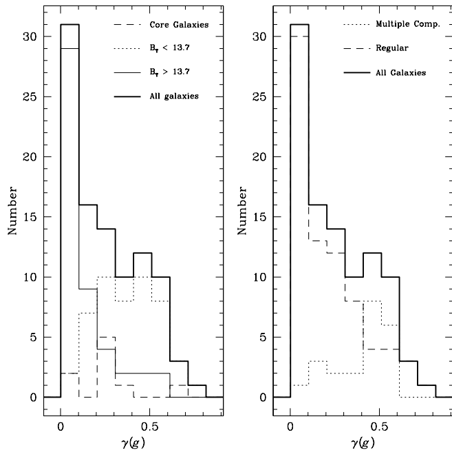
FIG. 118.—Distribution of the g -band inner slope \gamma of the galaxy profile (i.e., excluding a nuclear component) for the entire sample (shown by the solid line), and the sample divided according to their total B -band magnitude ( left panel ) and the presence of multiple morphological components ( right panel ). \gamma is measured from the best-fit profiles, and therefore represents the slope prior to PSF convolution and excluding a nuclear component. In the case of galaxies best fitted by a Sérsic profile, \gamma is measured at 0''.1 from the center following eq. (16).
