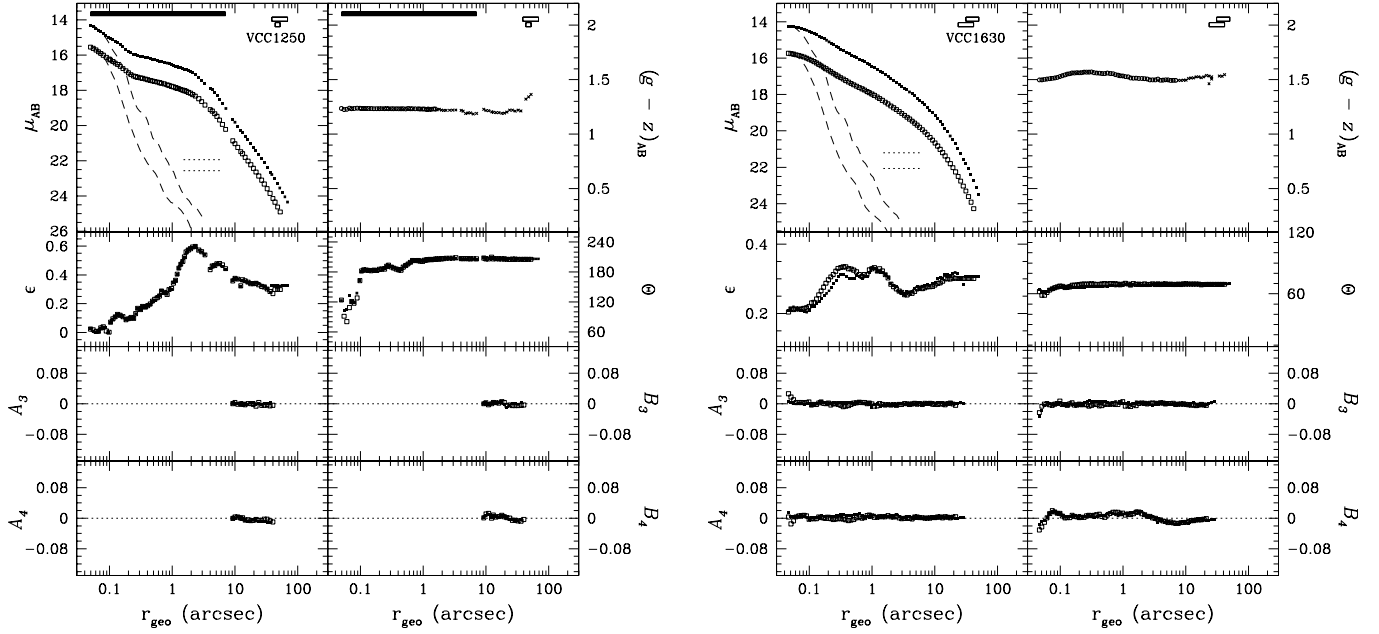
FIG. 69.— Left: VCC 1250 (=NGC 4476, Hubble type S0 3 (5)). Right: VCC 1630 (=NGC 4551, Hubble type E2). See Fig. 51 for details.
