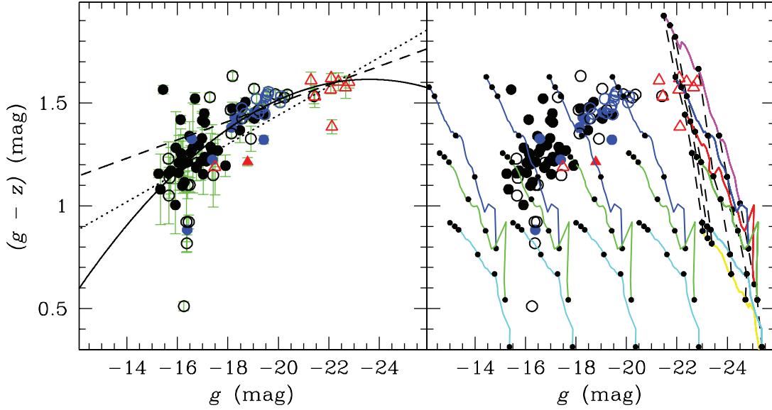
FIG. 123.—Color-magnitude diagram for the 100 galaxies that comprise the ACSVCS. Galaxies are color-coded as in Fig. 115. In the left panel, the data are plotted with error bars; the dashed and dotted lines corresponds to least-squares fits to galaxies fainter and brighter than M_g = -18 mag, respectively, while the curved line represents the best quadratic fit to the entire sample (see eqs. [31], [32], and [33]). The solid lines in the right panel show the prediction of the stellar population synthesis models of Bruzual & Charlot (2003). Models of constant metallicity and varying age are shown as solid lines for [\text{Fe}/\text{H}] = -2.25 (yellow), -1.65 (cyan), -0.64 (green), -0.33 (red), +0.09 (blue), +0.56 (magenta). Points along the isometallicity tracks corresponds to ages of 1, 2, 4, 8, 12, 15 Gyr (from left to right). Finally, from top to bottom, the g -band magnitudes have been scaled to a total mass M = 10^{12} , 10^{11} , 10^{10} , 10^9 , and 10^8 M_\odot . All magnitudes have been extinction corrected.
