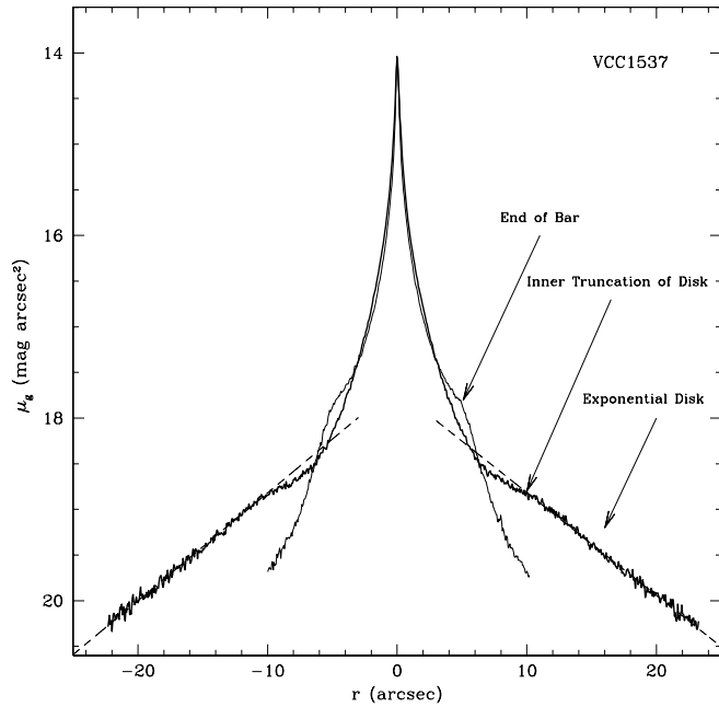
FIG. 109.— Cuts through the g -band photometric major axis ( thick solid line ) and through the bar axis ( thin solid line ) of VCC 1537 (NGC 4528)—the latter is misaligned by roughly 30^\circ relative to the minor axis of the galaxy. The inner truncation in the exponential disk (approximated by the dashed line), as well as the ends of the bar are marked.
