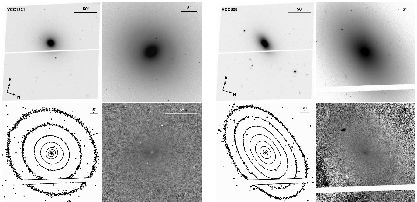
FIG. 18.— Left : VCC 1321 (=NGC 4489, Hubble type S0 1 (1)). Right : VCC 828 (=NGC 4387, Hubble type E5). See Fig. 1 for details.
