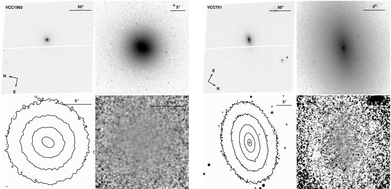
FIG. 44.— Left : VCC 1993 (Hubble type E0). Right : VCC 751 (=IC 3292, Hubble type dS0). See Fig. 1 for details.
