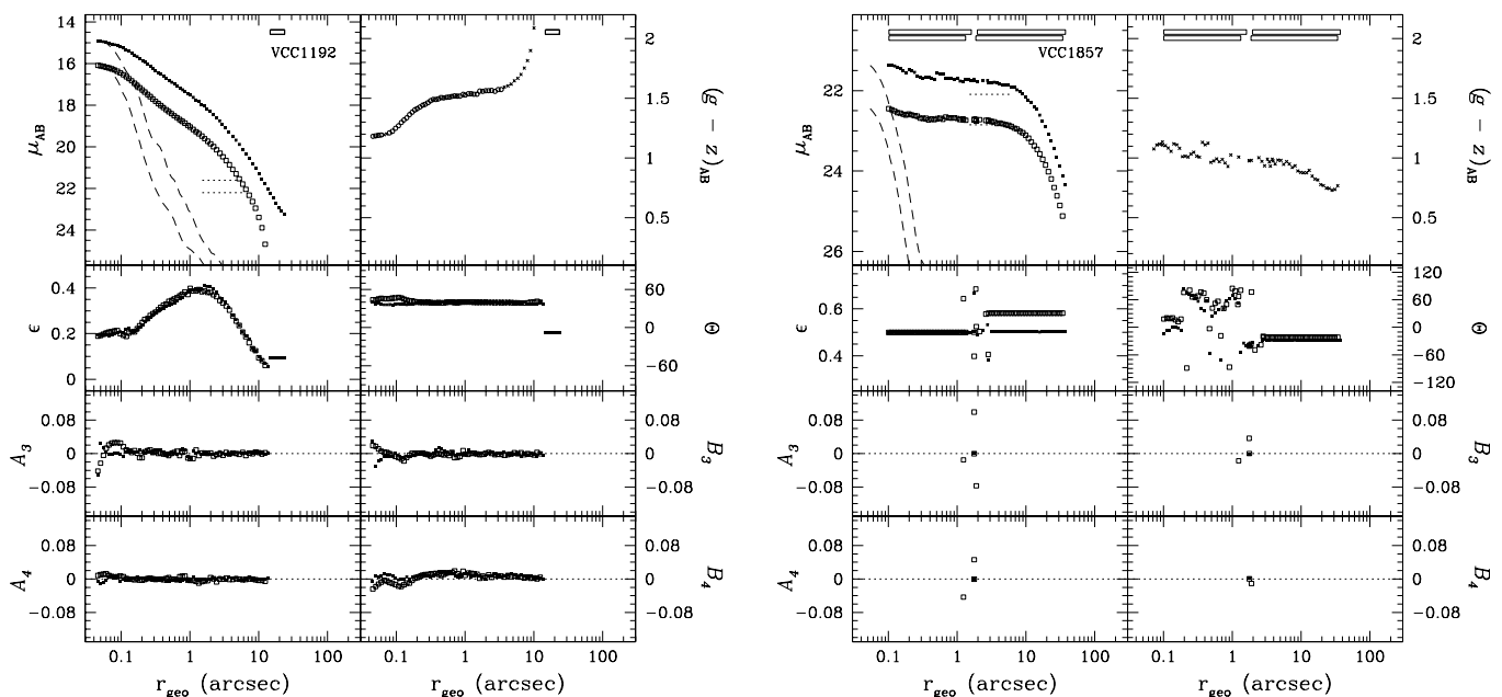
FIG. 90.— Left: VCC 1192 (=NGC 4467, Hubble type E3). Right: VCC 1857 (=IC 3647, Hubble type dE4:,N?). See Fig. 51 for details.
