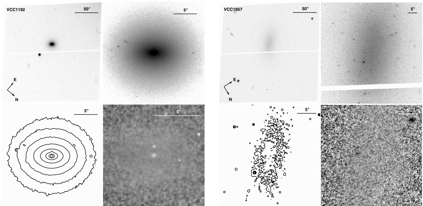
FIG. 40.— Left : VCC 1192 (=NGC 4467, Hubble type E3). Right : VCC 1857 (=IC 3647, Hubble type dE4:N?). See Fig. 1 for details.
