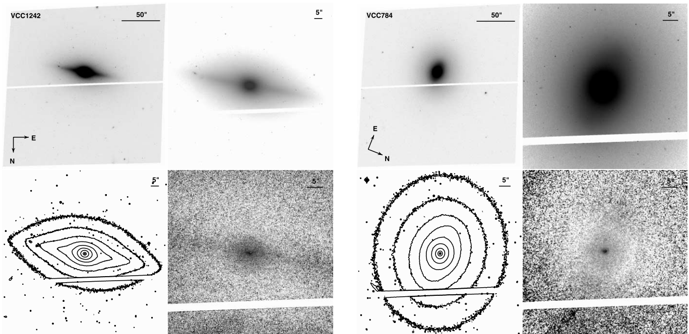
FIG. 16.— Left: VCC 1242 (=NGC 4474, Hubble type S0 1 (8)). Right: VCC 784 (=NGC 4379, Hubble type S0 1 (2)). See Fig. 1 for details.
