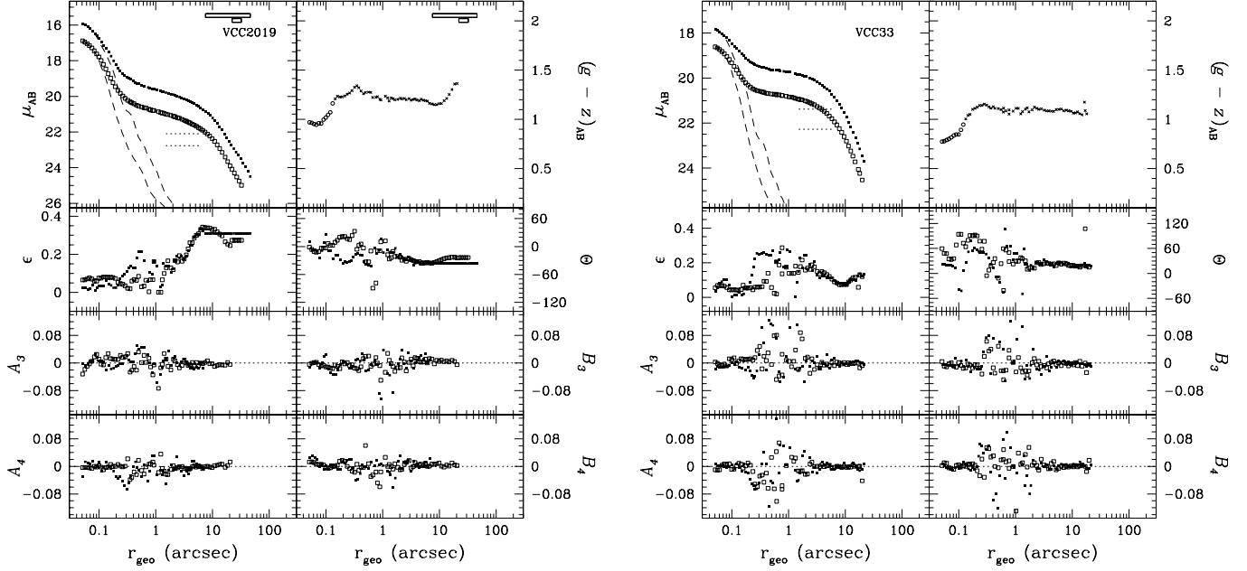
FIG. 85.— Left : VCC 2019 (=IC 3735, Hubble type dE4,N). Right : VCC 33 (=IC 3032, Hubble type d:E2,N:). See Fig. 51 for details.
