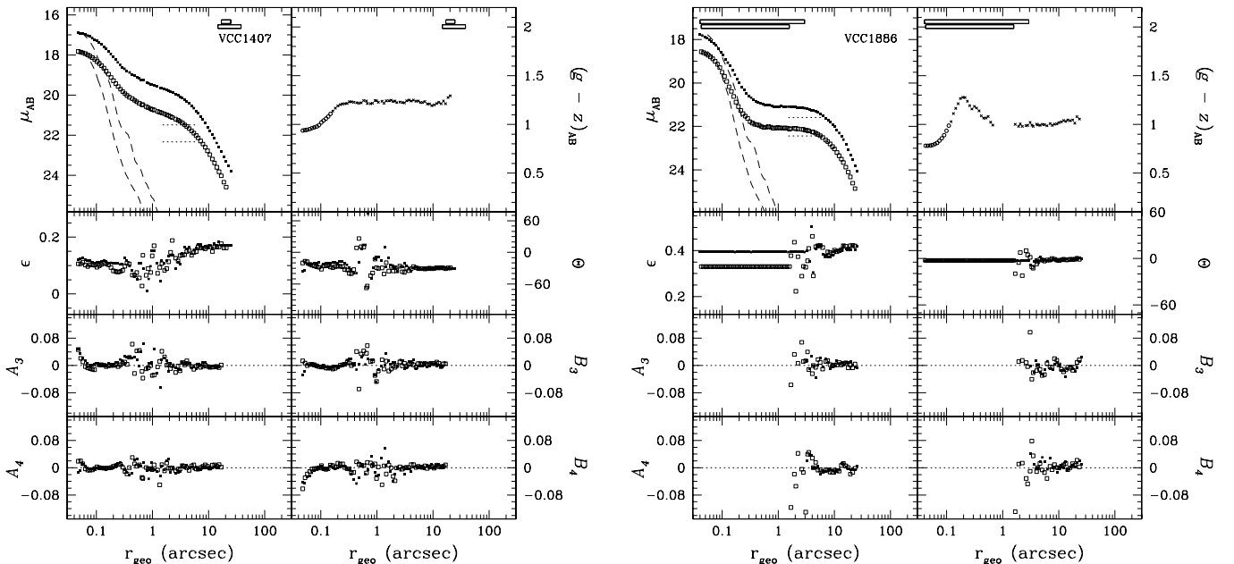
FIG. 96.— Left : VCC 1407 (=IC 3461, Hubble type dE2,N). Right : VCC 1886 (Hubble type dE5,N). See Fig. 51 for details.
