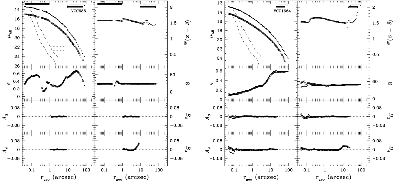
FIG. 61.— Left: VCC 685 (=NGC 4350, Hubble type S0 1 (8)). Right: VCC 1664 (=NGC 4564, Hubble type E6). See Fig. 51 for details.
