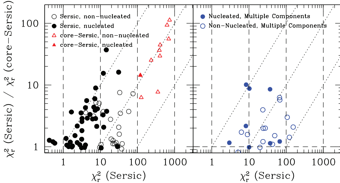
FIG. 113.—Ratio of the reduced \chi^2 of the Sérsic and core-Sérsic fits vs. the reduced \chi^2 for the best Sérsic fit (see text for details). Galaxies with stellar disks or bars are shown in the right panel, “regular” galaxies in the left panel. The dotted lines represent loci for which (from left to right) \chi_r^2(\text{core-Sérsic}) = 1, 10, 100 ; the dashed lines have the same meaning for \chi_r^2(\text{Sérsic}) . Galaxies plotted as triangles are best fitted by a core-Sérsic profile.
