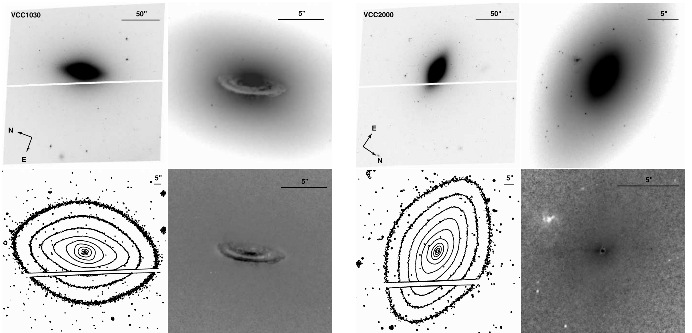
FIG. 10.— Left : VCC 1030 (=NGC 4435, Hubble type SB0 1 (6)). Right : VCC 2000 (=NGC 4660, Hubble type E3/S0 1 (3)). See Fig. 1 for details.
