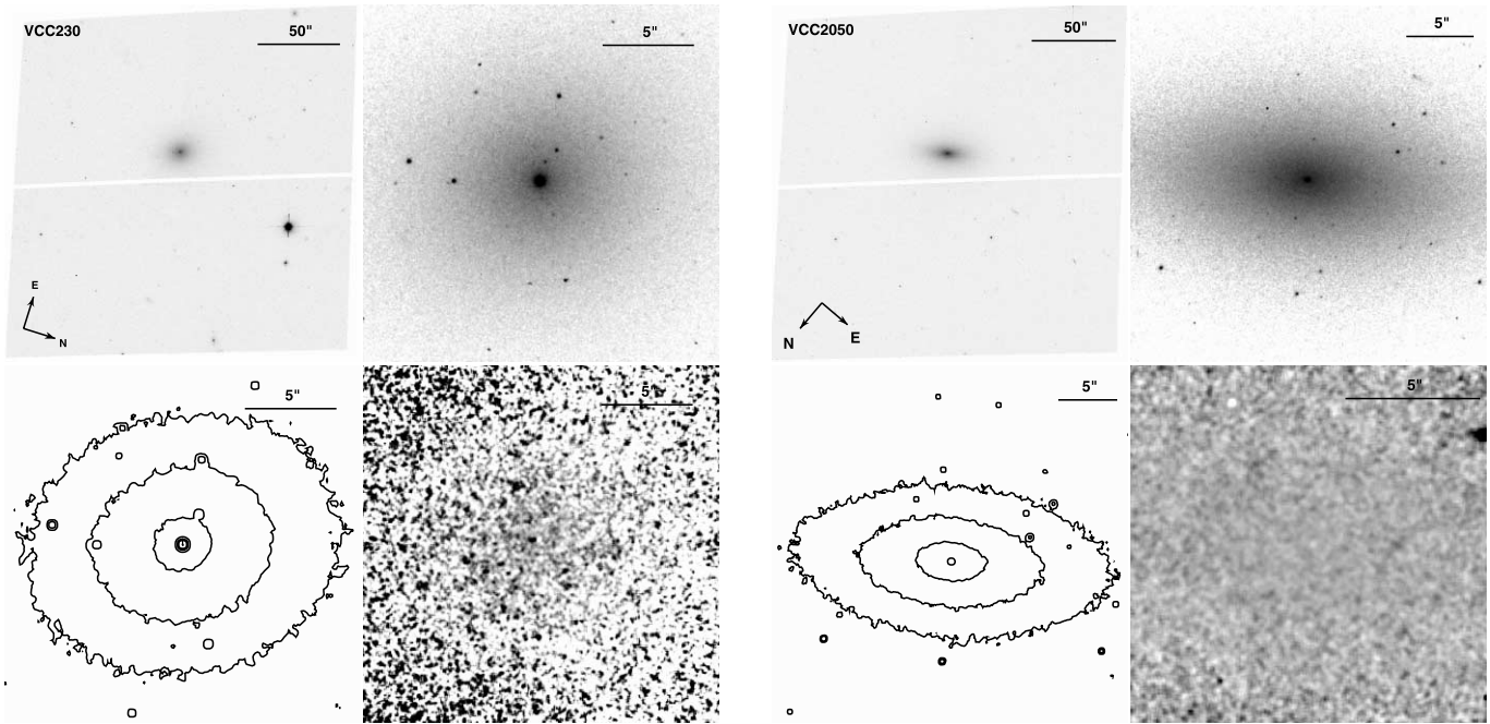
FIG. 43.— Left : VCC 230 (=IC 3101, Hubble type dE4+,N:). Right : VCC 2050 (=IC 3779, Hubble type dE5+,N). See Fig. 1 for details.
