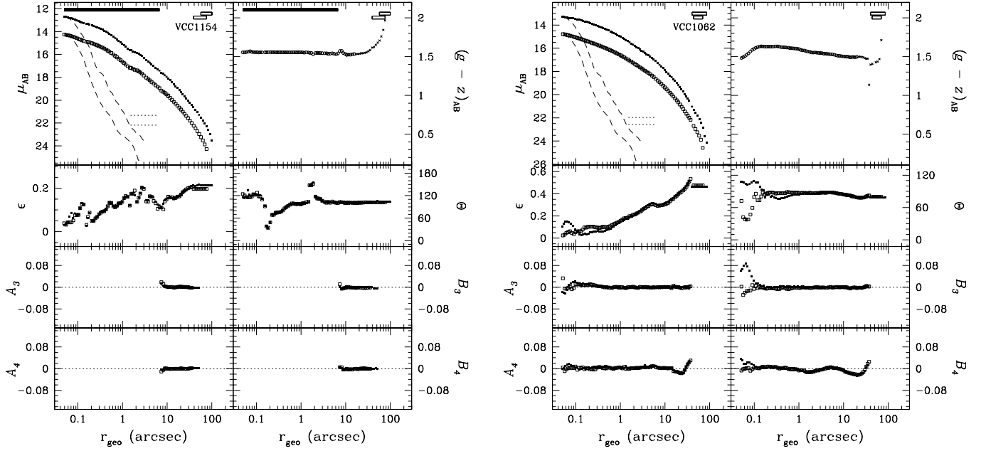
FIG. 57.— Left : VCC 1154 (=NGC 4459, Hubble type S0 3 (2)). Right : VCC 1062 (=NGC 4442, Hubble type SB0 1 (6)). See Fig. 51 for details.
