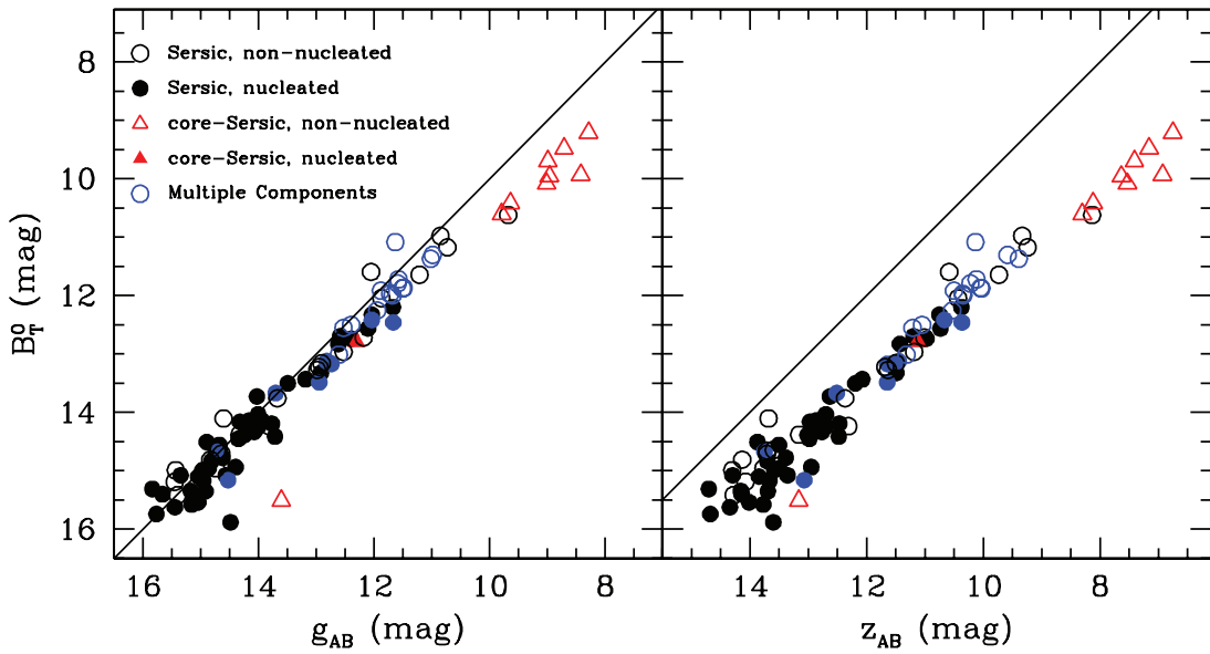
FIG. 115.— Comparison of the g - and z -band total magnitudes, corrected for extinction, derived by integrating to infinity the best-fitting surface brightness profiles, compared to the B_T^g magnitudes from the RC3. The diagonal line shows a one-to-one correspondence. Galaxies with multiple morphological components, for which the model fits are not always satisfactory, are plotted in blue.
