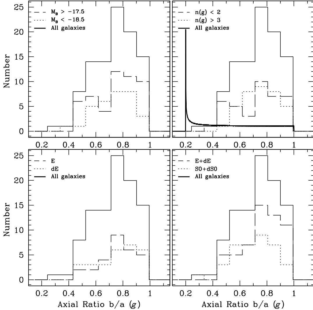
FIG. 122.—The distribution of minor to major axes ratios, b/a , for the ACSVCS galaxies. In all panels, the thick solid line shows the distribution for the entire sample. In the upper left and right panels the sample is divided according to absolute B -band magnitude and Sérsic index n , respectively; the thick continuous line in the right panel shows the distribution of axial ratios expected for a population of galaxies with intrinsic b/a = 0.2 and seen at random orientations. In the bottom left and right panels, the sample is divided according to morphological classification.
