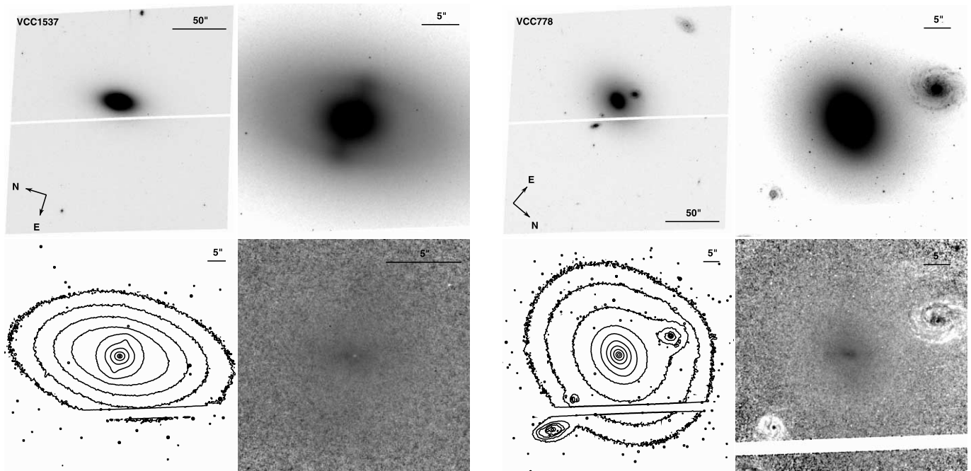
FIG. 17.— Left : VCC 1537 (=NGC 4528, Hubble type SB0 2 (5)). Right : VCC 778 (=NGC 4377, Hubble type S0 1 (3)). See Fig. 1 for details.
