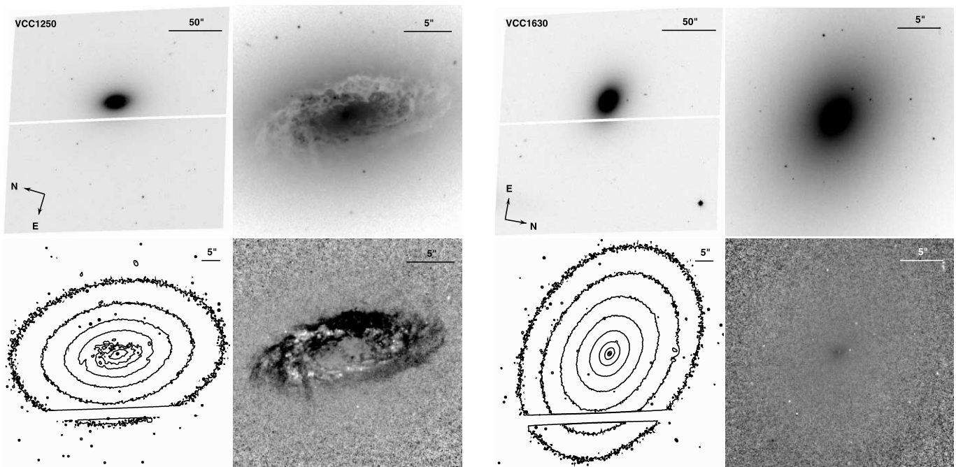
FIG. 19.— Left : VCC 1250 (=NGC 4476, Hubble type S0_3(5) ). Right : VCC 1630 (=NGC 4551, Hubble type E2). See Fig. 1 for details.
