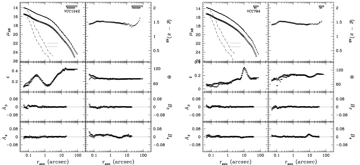
FIG. 66.— Left: VCC 1242 (=NGC 4474, Hubble type S0 1 (8)). Right: VCC 784 (=NGC 4379, Hubble type S0 1 (2)). See Fig. 51 for details.
