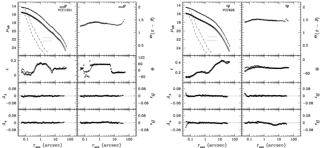
FIG. 68.—Left: VCC 1321 (=NGC 4489, Hubble type S0 1 (1)). Right: VCC 828 (=NGC 4387, Hubble type E5). See Fig. 51 for details.
