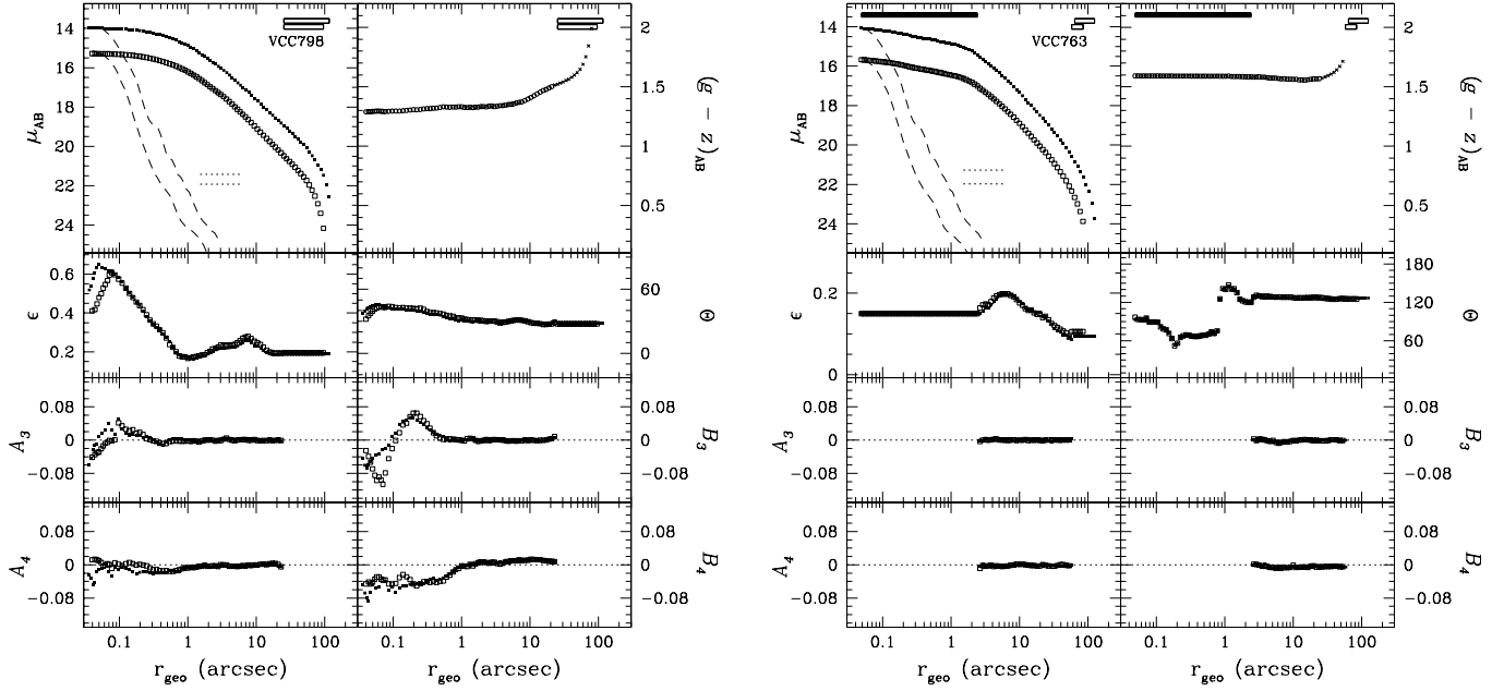
FIG. 53.— Left: VCC 798 (=M85, NGC 4382, Hubble type S0 1 (3) pec). Right: VCC 763 (=M84, NGC 4374, Hubble type E1). See Fig. 51 for details.
