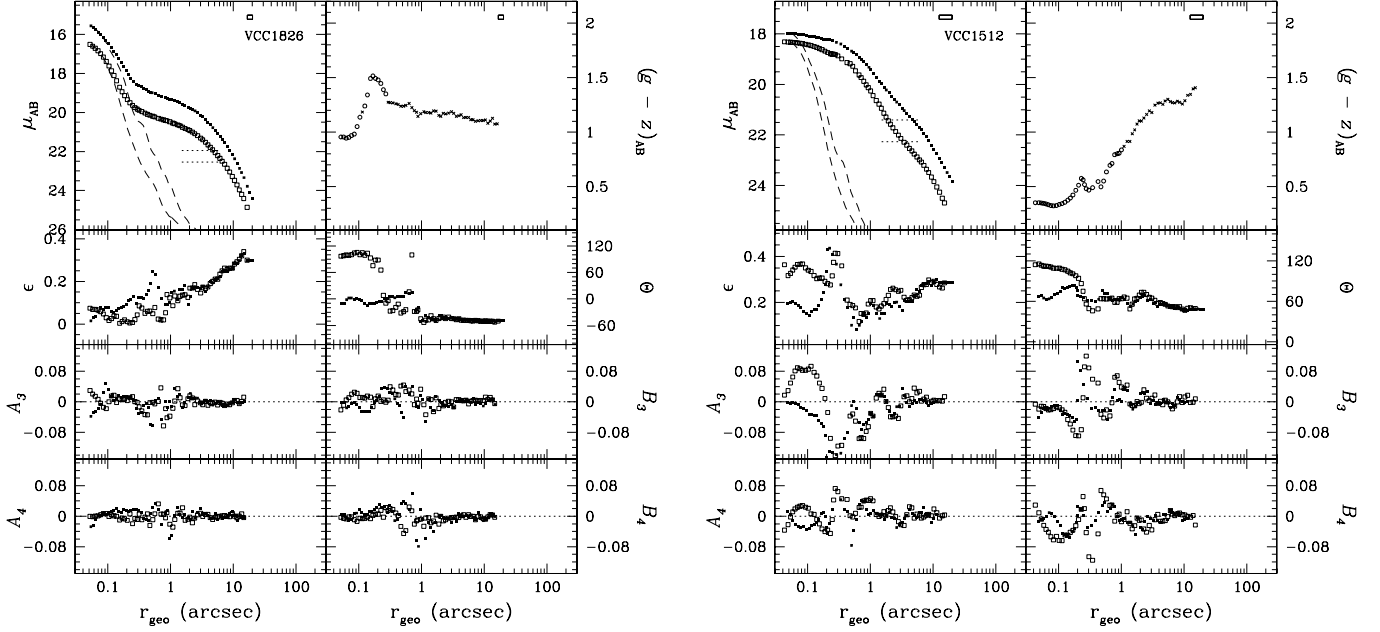
FIG. 99.— Left : VCC 1826 (=IC 3633, Hubble type dE2,N). Right : VCC 1512 (Hubble type dS0 pec). See Fig. 51 for details.
