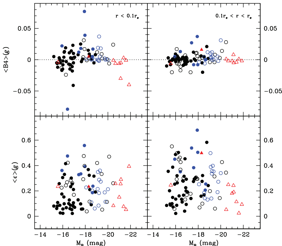
FIG. 121.—Correlations between the extinction-corrected B -band magnitude and mean ellipticity and B4 coefficients. The latter are calculated within 10% of the effective radius r_e (excluding the nuclear region, if a nucleus is present) in the left panels, and between 0.1r_e and r_e in the panels to the right. Galaxies are color-coded as in the legend of Fig. 115, blue points refer to galaxies with multiple morphological components.
