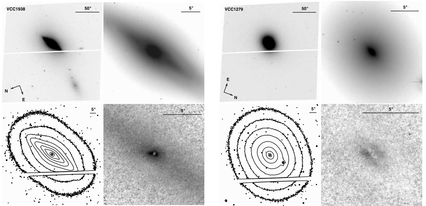
FIG. 13.— Left : VCC 1938 (=NGC 4638, Hubble type S0_1(7) ). Right : VCC 1279 (=NGC 4478, Hubble type E2). See Fig. 1 for details.
