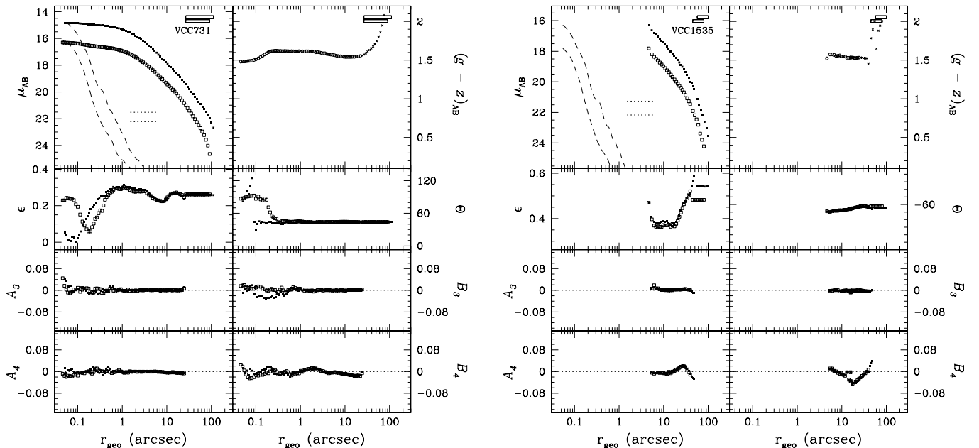
FIG. 54.— Left: VCC 731 (=NGC 4365, Hubble type E3). Right: VCC 1535 (=NGC 4526, Hubble type S0 3 (6)). See Fig. 51 for details.
