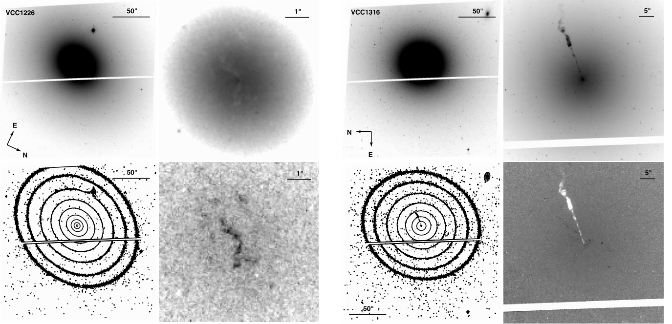
FIG. 1.— Left : The ACSVCS g -band image for VCC 1226 (=M49; NGC 4472, Hubble type E2/S01(2), see Table 1), the first ranked member of Virgo. The top panels show the ACS/WFC/F475W full frame ( left panel ) and a zoom toward the center ( right panel ); the gray-scale used for the top left panel (full frame) is kept the same in Figs. 1–50; while the gray-scale for the top right panel changes from galaxy to galaxy. The bottom left panel shows a contour map of the g -band frame, with levels drawn (here and for all subsequent galaxies) at 0.05, 0.1, 0.2, 0.4, 0.8, 1.6, 3.2, 6.4, 12.8, 25.6 electrons \text{s}^{-1} \text{pixel}^{-1} (22.82 mag \text{arcsec}^{-2} to 16.04 mag \text{arcsec}^{-2} , see eq. [4]). Finally, the bottom right panel shows a central section of the g - z color image, with red regions appearing as dark areas and blue regions as light. The linear scale is shown in each panel. All images have been background subtracted. Right : As at left, but for VCC 1316 (=M87; NGC 4486, Hubble type E0).
