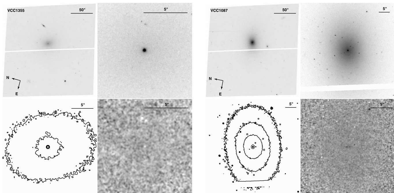
FIG. 30.— Left : VCC 1355 (=IC 3442, Hubble type dE2,N). Right : VCC 1087 (=IC 3381, Hubble type dE3,N). See Fig. 1 for details.
