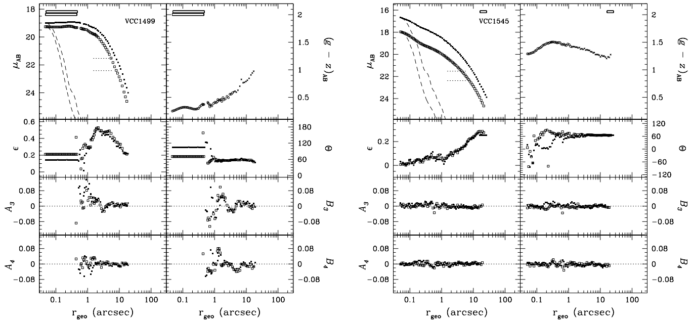
FIG. 89.— Left: VCC 1499 (=IC 3492, Hubble type E3 pec or S0). Right: VCC 1545 (=IC 3509, Hubble type E4). See Fig. 51 for details.
