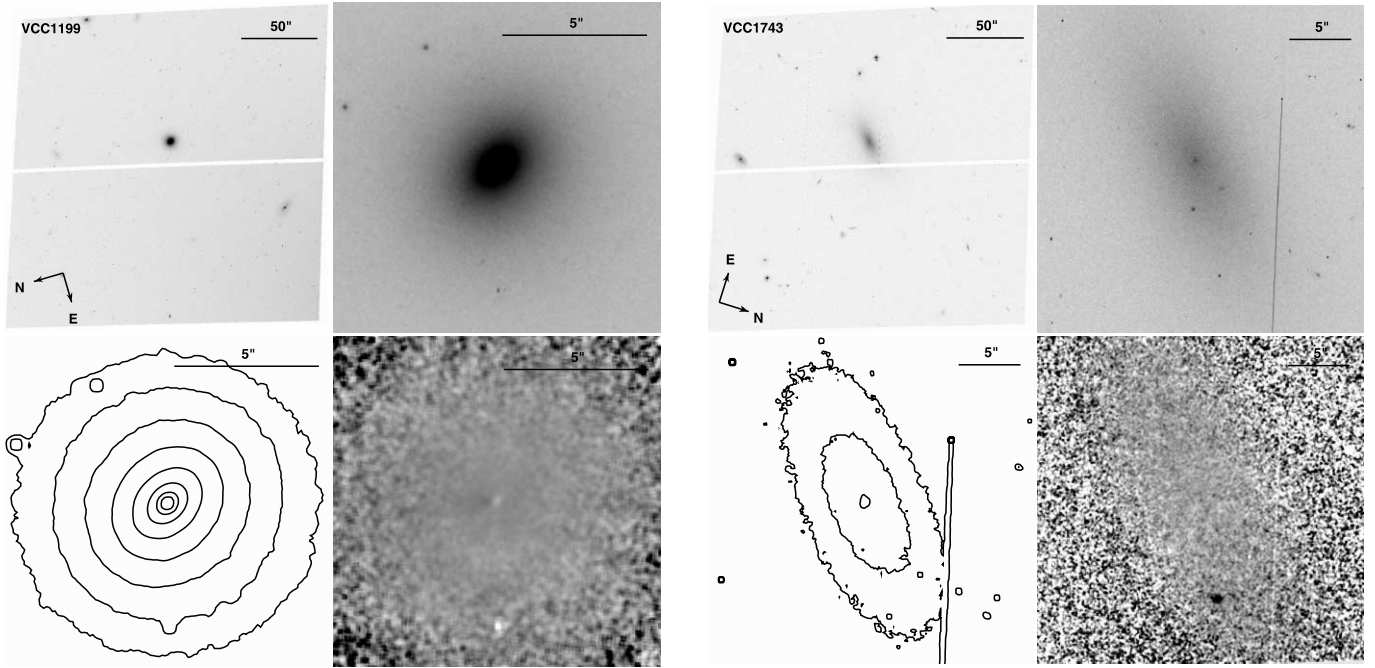
FIG. 47.— Left : VCC 1199 (Hubble type E2). Right : VCC 1743 (=IC 3602, Hubble type dE6). See Fig. 1 for details.
