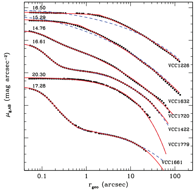
FIG. 111.— Representative g -band surface brightness profiles for six galaxies in the ACS Virgo Cluster Survey, from the brightest (VCC 1226) to the faintest (VCC 1661) galaxy in the sample, plotted as a function of the geometric mean radius. All galaxies are “regular” ellipticals, in the sense of not displaying significant morphological peculiarities (with the exception of the possible presence of a nuclear component). The galaxies are arranged, from top to bottom, in order of increasing total B -band magnitude (decreasing luminosity). They have been shifted in the vertical direction for clarity; the value of the g -band surface brightness profile at 0''.049 is listed on the left-hand side next to each galaxy profile, and tic marks on the ordinate axis are separated by 1 \text{ mag arcsec}^{-2} . For each galaxy, we overplot the best-fit Sérsic ( dashed line ) and core-Sérsic ( solid line ) model, with addition of a King model for nucleated galaxies (VCC 1720, VCC 1422 and VCC 1661).
