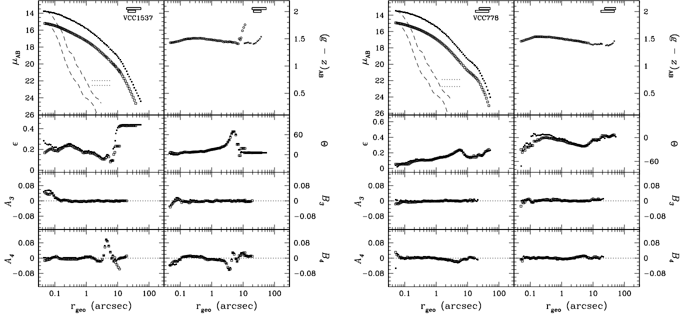
FIG. 67.—Left: VCC 1537 (=NGC 4528, Hubble type SB 0 (5)). Right: VCC 778 (=NGC 4377, Hubble type S0 1 (3)). See Fig. 51 for details.
