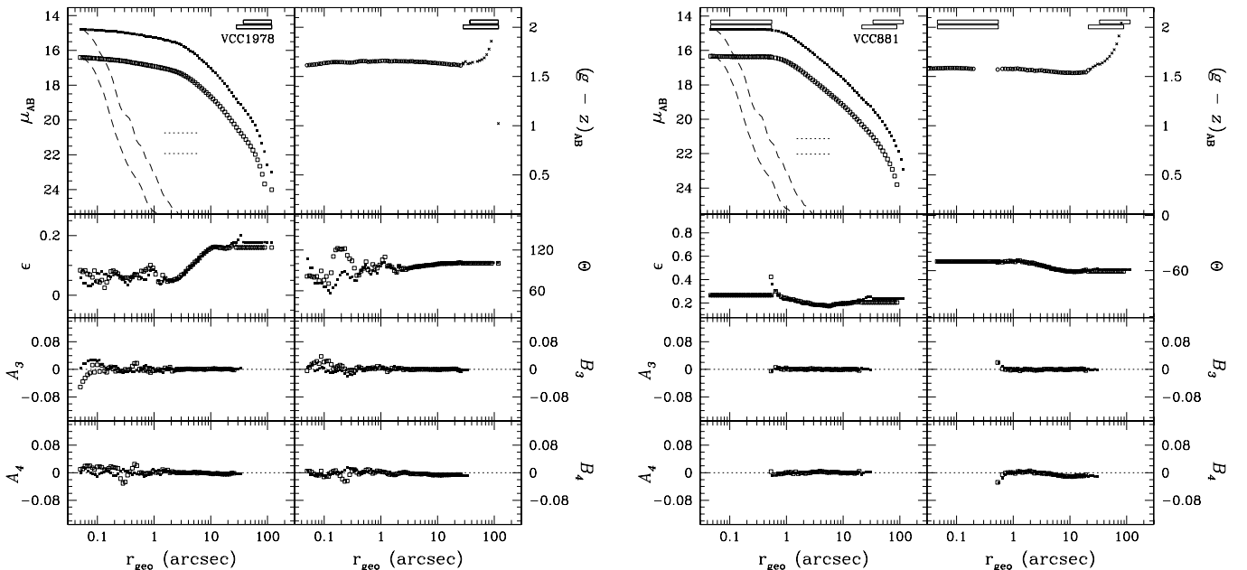
FIG. 52.— Left : VCC 1978 (=M60, NGC 4649, Hubble type S0 _1 (2)). Right : VCC 881 (=M86, NGC 4406, Hubble type S0 _1 (3)/E3). See Fig. 51 for details.
