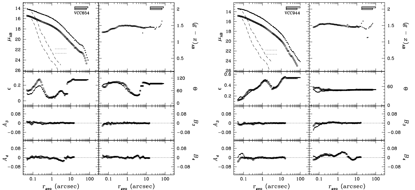
FIG. 62.— Left: VCC 654 (=NGC 4340, Hubble type RSB0 2 (5)). Right: VCC 944 (=NGC 4417, Hubble type S0 1 (7)). See Fig. 51 for details.
