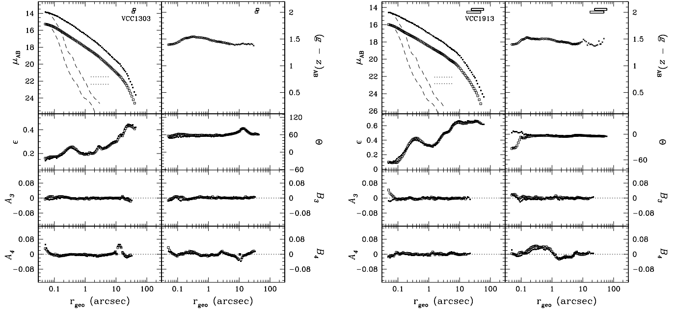
FIG. 71.— Left: VCC 1303 (=NGC 4483, Hubble type SB0 1 (5)). Right: VCC 1913 (=NGC 4623, Hubble type E7). See Fig. 51 for details.
