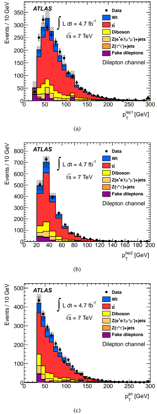
Figure 2: Kinematic distributions comparing data to predictions in the dilepton channel for (a) the leading lepton p_T^{\text{lep1}} , (b) the sub-leading lepton p_T^{\text{lep2}} and (c) the jet p_T^{\text{jet}} . The hatched band shows the uncertainty due to the background normalisation. The last bin includes overflows.
