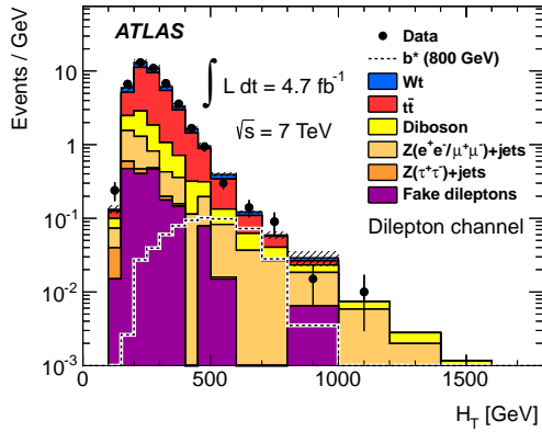
Figure 3: H_T distribution for data and background expectation for the dilepton channel. The hatched band shows the uncertainty due to the background normalisation. The signal for a b^* -quark mass of 800 GeV is also shown.
