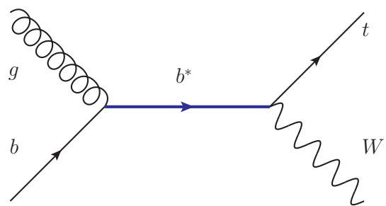
Figure 1: Leading-order Feynman diagram for single- b^* -quark production and decay to Wt .
