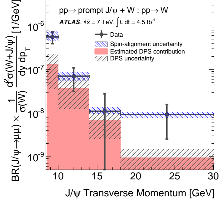
Figure 6. The inclusive (SPS+DPS) cross-section ratio dR_{J/\psi}^{\text{incl}}/dp_T is shown as a function of J/\psi transverse momentum. The shaded uncertainty corresponds to the variations due to the various spin-alignment scenarios. The DPS estimate is overlaid, with the uncertainty again shown by a shaded region.
