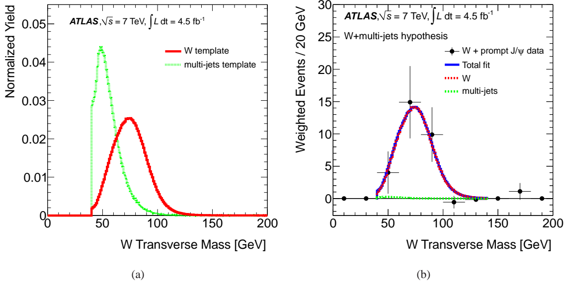
Figure 3. (a) Unit-normalized templates for W boson transverse mass m_T(W) for multi-jet background and W^\pm boson signal. (b) sPlot-weighted W boson transverse mass distribution for W^\pm + \text{prompt } J/\psi candidate events with a fit to the W^\pm boson and multi-jet components. The fit is performed in the region 40–140 GeV in m_T(W) .
