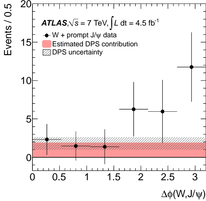
Figure 4. The sPlot-weighted azimuthal angle between the W^\pm and the J/\psi is shown for W^\pm + prompt J/\psi candidates. No efficiency or acceptance corrections are applied. The determined DPS contribution (with systematic uncertainties) is overlaid, using a flat DPS template validated using PYTHIA8 [44] Monte Carlo simulation and normalized to the total rate as estimated using the DPS ansatz in eq. 1. The hashed region shows the uncertainty on the DPS estimate.
