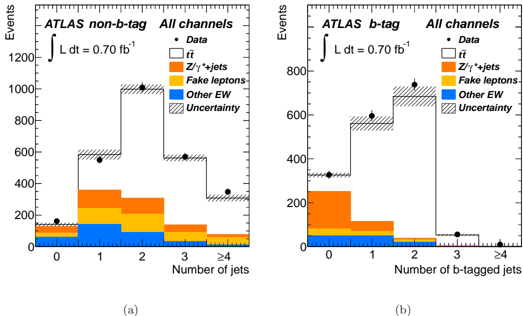
Figure 1. (a) Jet multiplicity distribution for ee+\mu\mu+e\mu+e\tau L+\mu\tau L events without a b -tagging requirement. (b) Multiplicity distribution of b -tagged jets in the ee+\mu\mu+e\mu channels. Contributions from diboson and single top-quark events are summarized as ‘Other EW’. The events in (b) are not a simple subset of those in (a) because the event selections for the b -tag and non- b -tag analyses differ. Uncertainties shown are statistical and systematic combined. The distributions are shown as stacked histograms.
