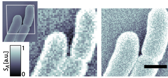
FIG. 2. (Upper left insert) High-resolution SEM image of fixated E. Coli . Brighter (darker) regions correlate with high (low) spin density. (Main images) Simulated “raster scan” reconstructions of the corresponding two-dimensional (2D) spin lattice. The color code gauges the average NV center fluorescence as determined after N_A observations during which the spin alignment changes randomly [see Eq. (10)]. The darker regions between and on the surface of the bacteria are artifacts resulting from artificial shadowing of the source SEM image. The tip-NV center distance and raster scan resolution is 30 nm (left) and 15 nm (right). The scale bar corresponds to 300 nm. Other parameters are as listed in the text.
