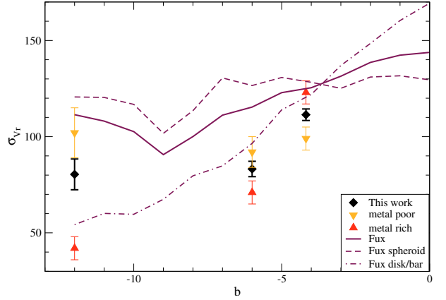
Fig. 8. Radial velocity dispersion along the bulge minor axis compared with the model of Fux (1999). The metal-poor and metal-rich population are defined by the 33% and 66% quantile of the [\text{Fe}/\text{H}] distribution.
