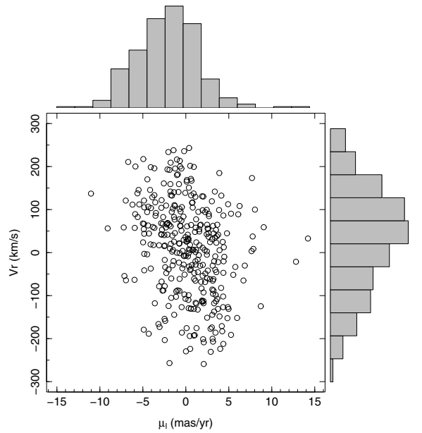
Fig. 2. V_r and \mu_l distributions in Baade’s Window.
