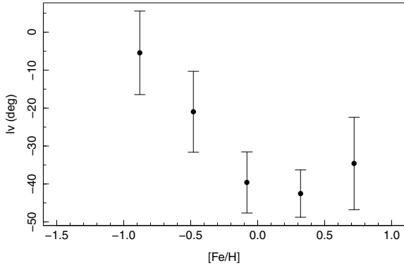
Fig. 3. Vertex deviation l_v in Baade’s Window as a function of metallicity by bins of 0.4 dex.
