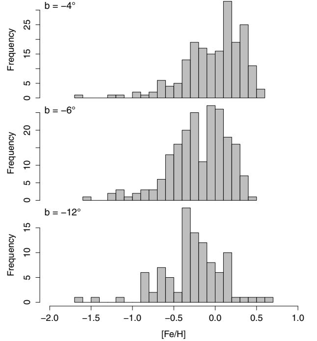
Fig. 5. Distribution of the metallicity for the different galactic latitudes of Paper I.
