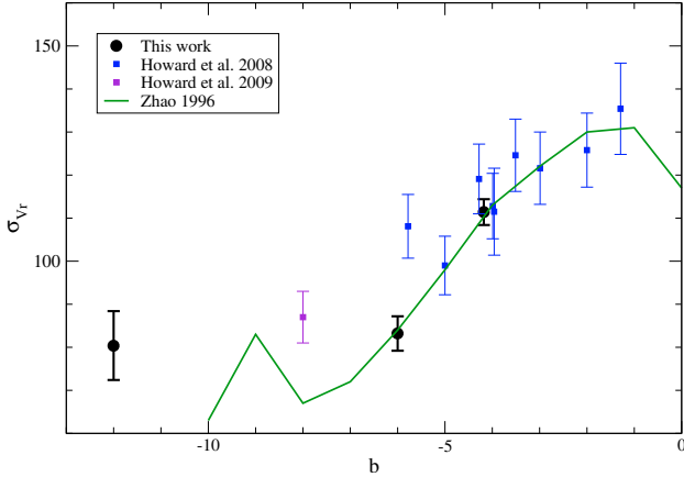
Fig. 7. Radial velocity dispersion along the bulge minor axis compared to the BRAVA data (Howard et al. 2008, 2009) and the model of Zhao (1996).
