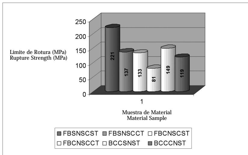
Figura 3. Comportamiento del Limite de Rotura Figure 3. Behavior of the rupture strength
